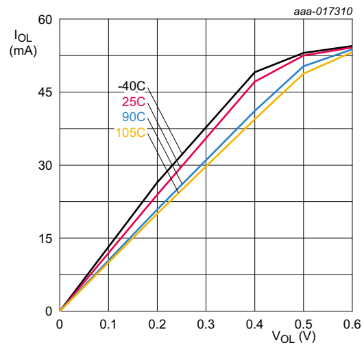
Fig 18. I 2 C-bus pins (high current sink): Typical LOW-level output current I_{OL} versus LOW-level output voltage V_{OL}
