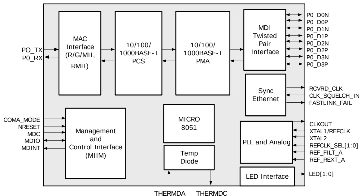
Figure 2 • Block Diagram
