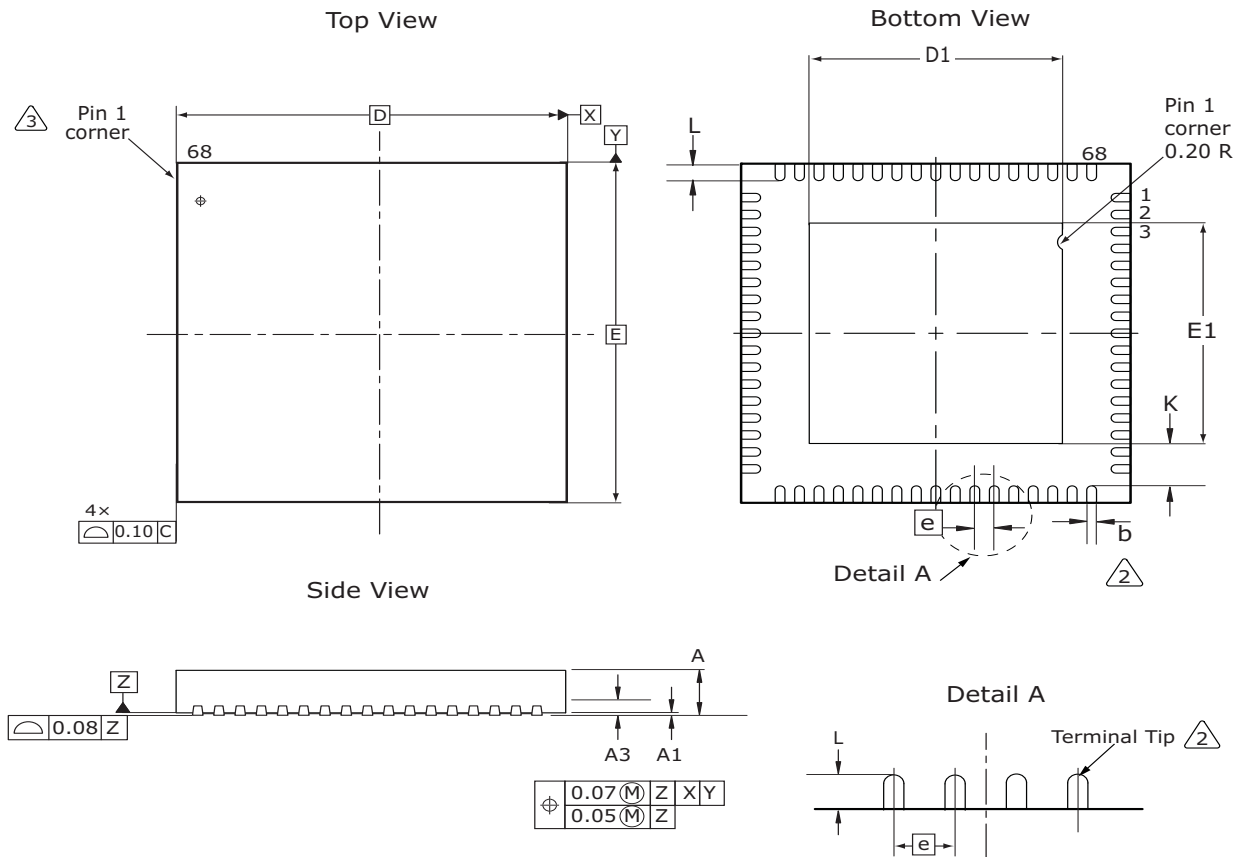
Figure 36 • Package Drawing
