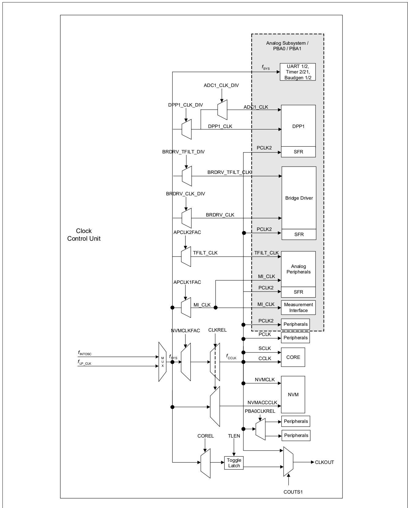
Figure 12 Clock Generation from f_{\text{sys}} ; CLKOUT Generation
