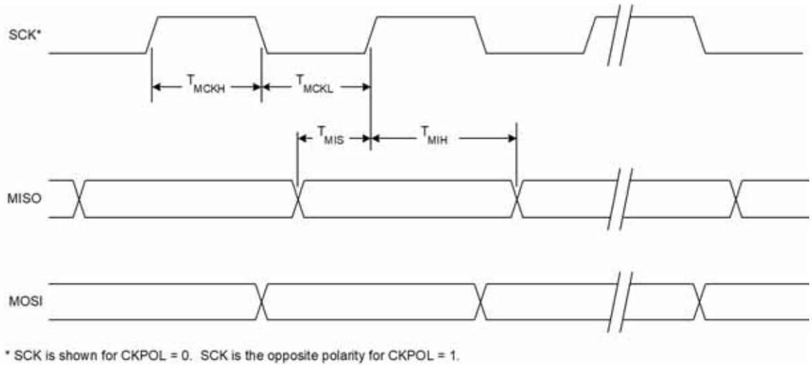
Figure 23.6. SPI Master Timing (CKPHA = 0)
