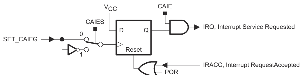
Figure 21-5. Comparator_A+ Interrupt System
