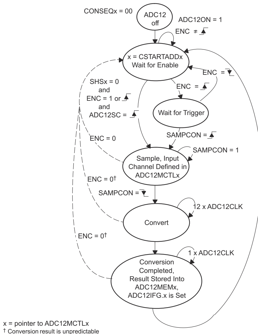
Figure 23-6. Single-Channel, Single-Conversion Mode
