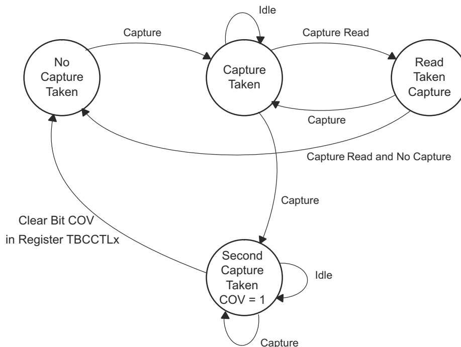
Figure 13-11. Capture Cycle
