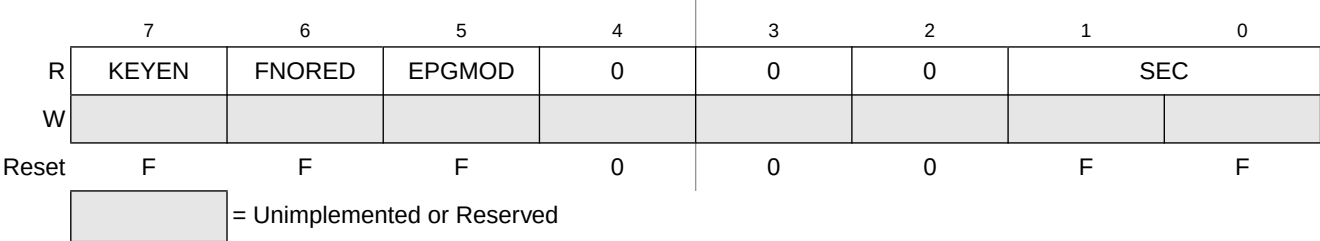
Figure 4-15. FLASH and EEPROM Options Register (FOPT)
