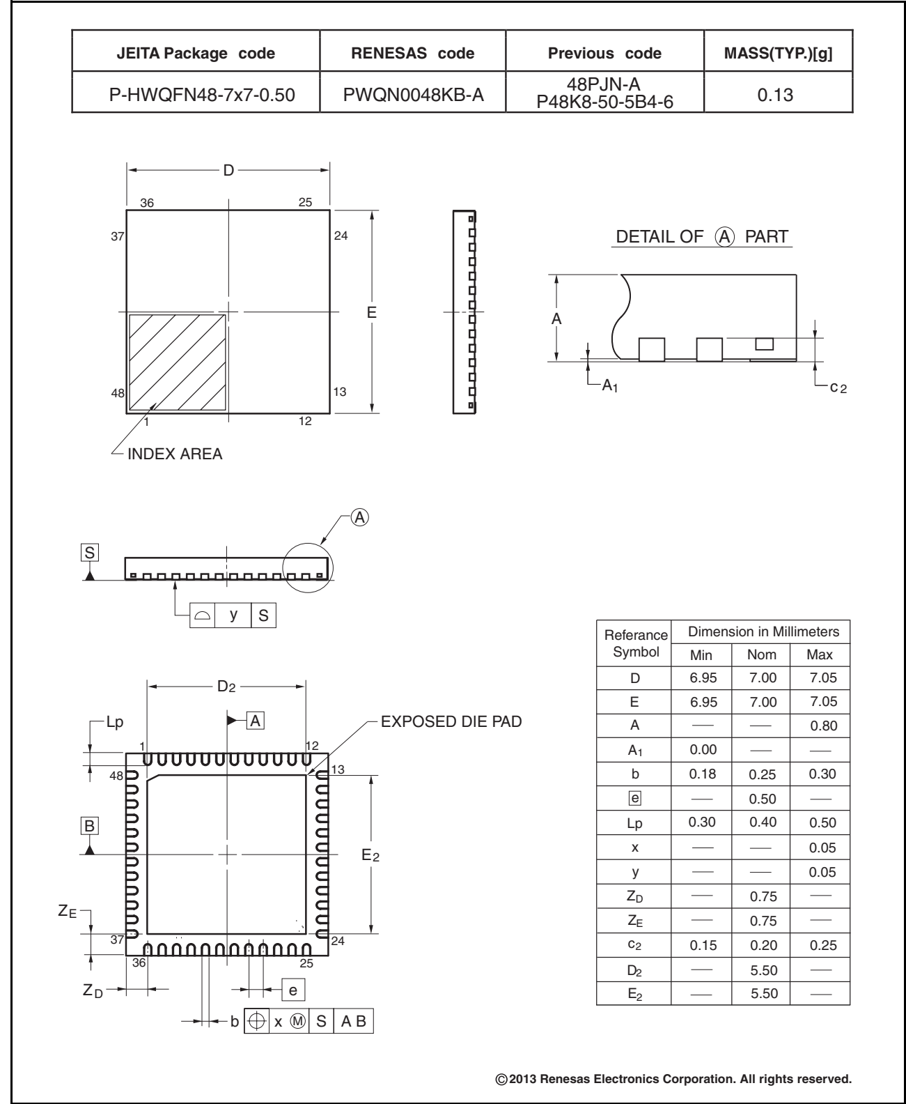
Figure 2.4 QFN 48-pin (1)
