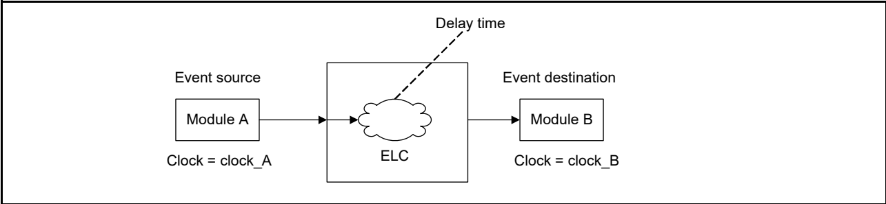
Figure 17.2 ELC delay time
