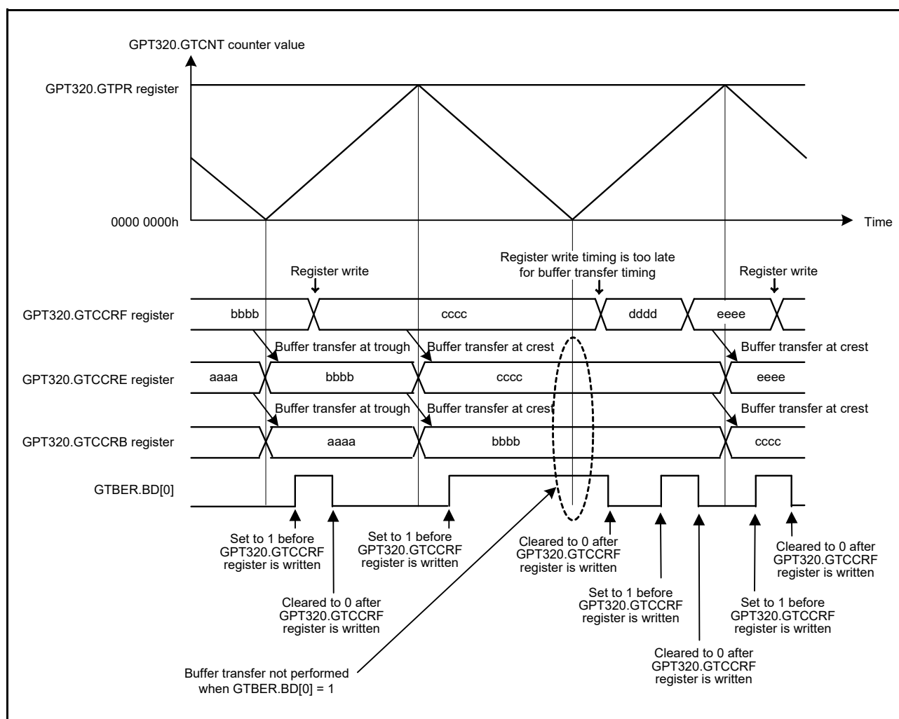
Figure 21.83 Example of operation for disabling buffer operation with triangle waves, double buffer operation, and buffer transfer at both troughs and crests
