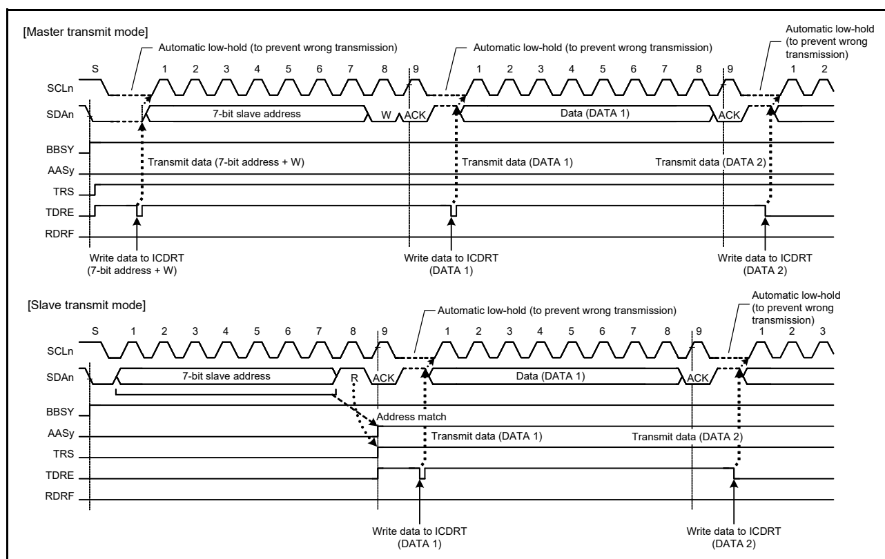
Figure 28.38 Automatic low-hold operation in transmit mode
