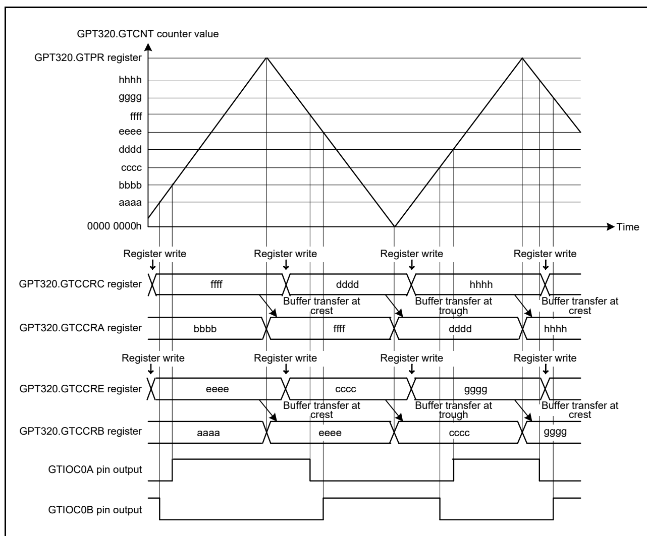
Figure 21.35 Example of triangle-wave PWM mode 2 operation with buffer operation, low output from the GTIOCA pin and high output from the GTIOCB pin at count start, output toggled at GTCCRA/GTCCRB compare match, and output retained at cycle end
