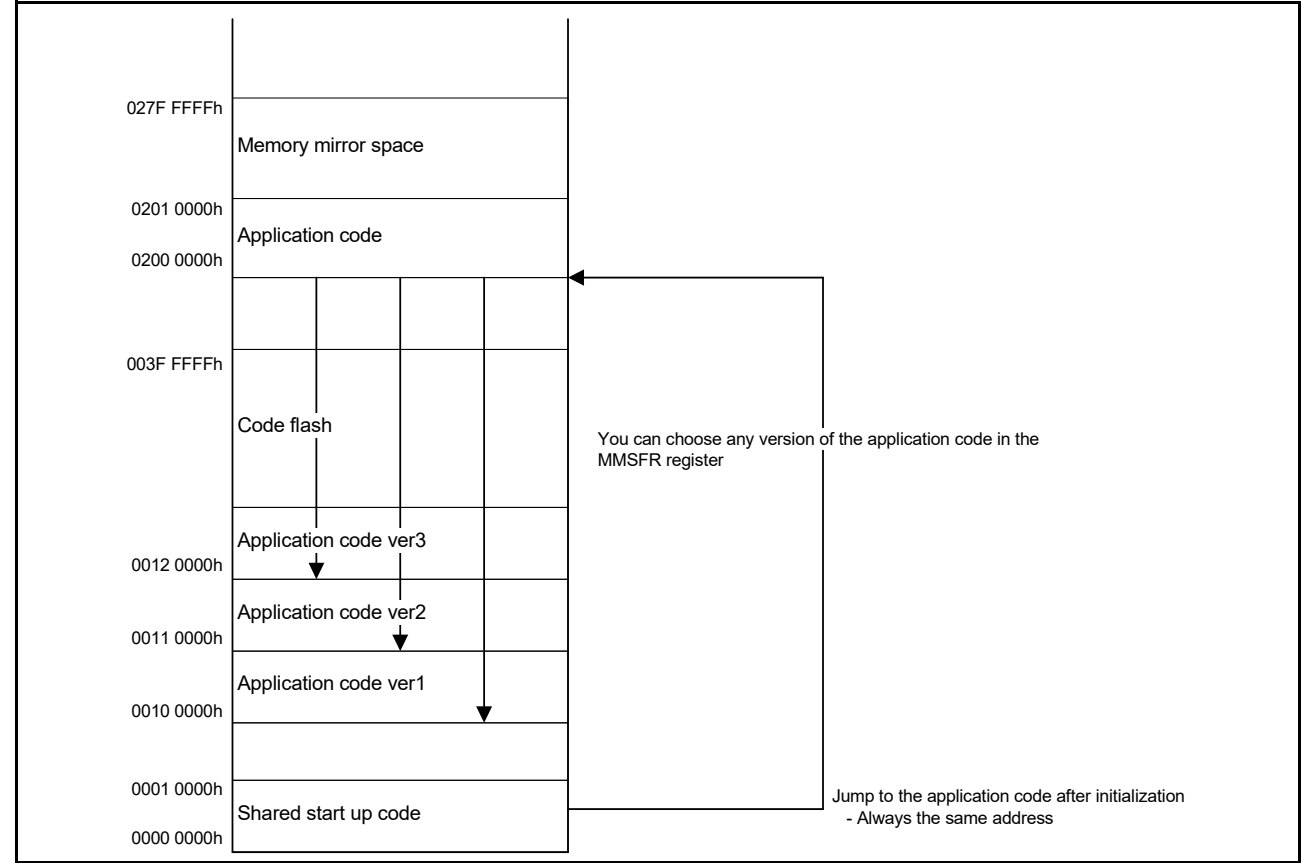
Figure 5.6 MMF setting example
