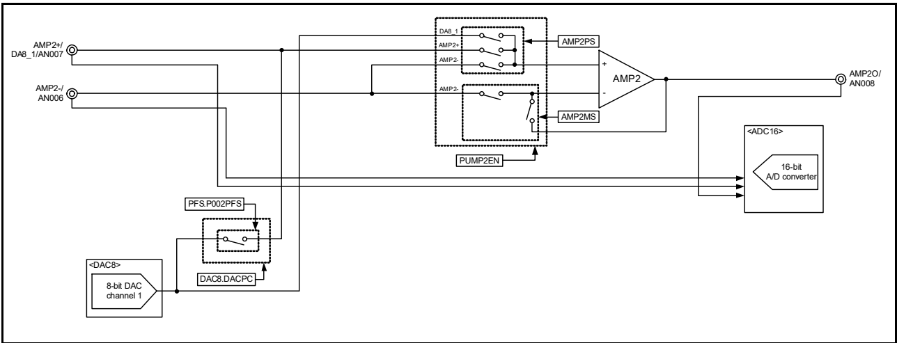
Figure 37.4 OPAMP2 block diagram
