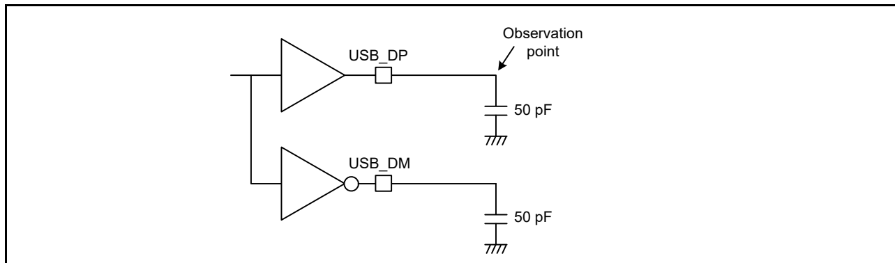
Figure 47.60 Test circuit for Full-Speed (FS) connection
