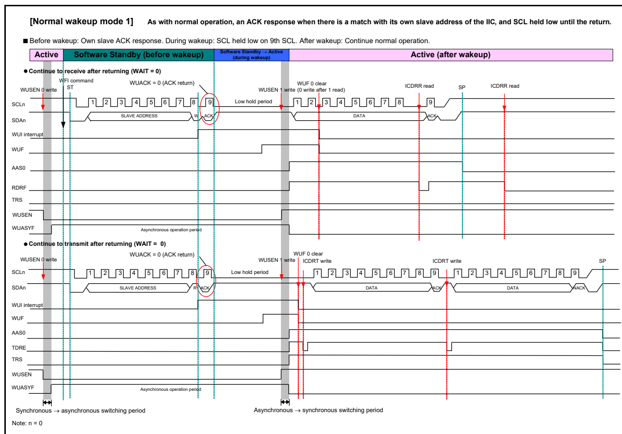
Figure 28.32 Timing of normal wakeup mode 1
