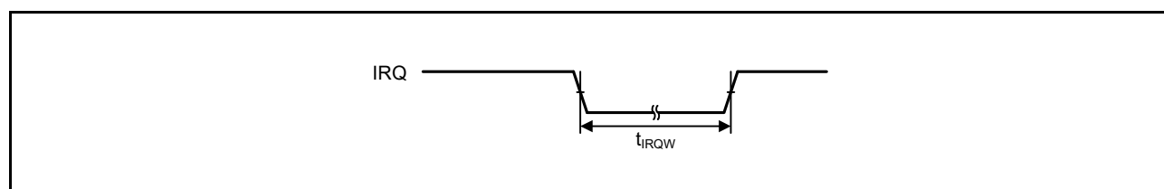
Figure 47.35 IRQ interrupt input timing
