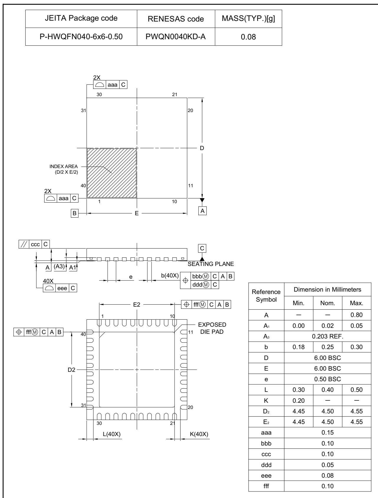
Figure 2.7 QFN 40-pin (2)
