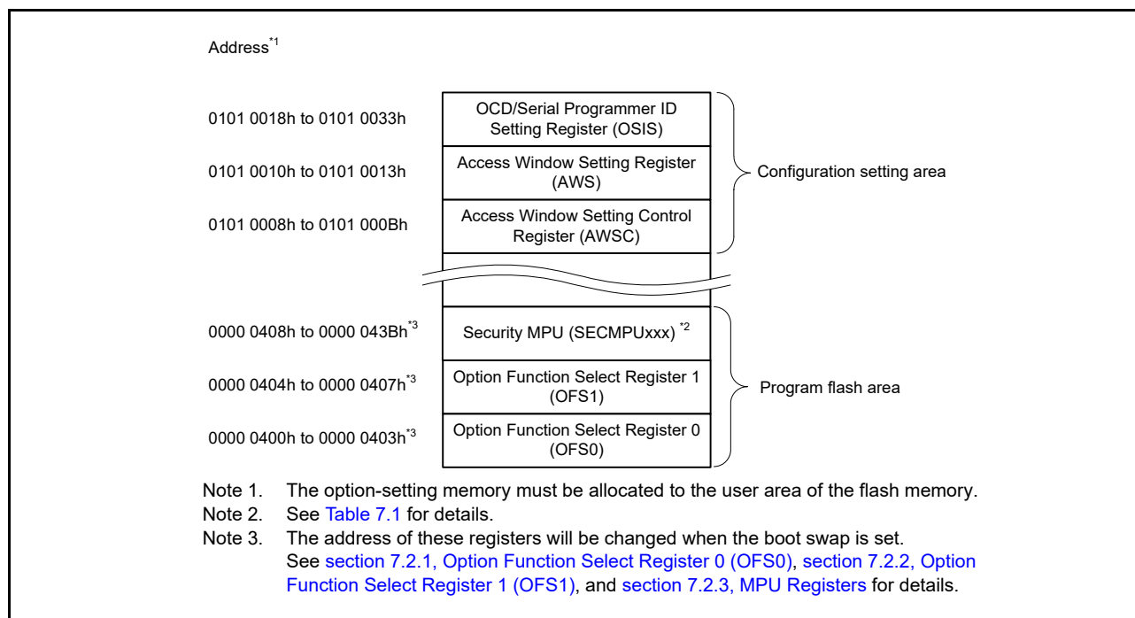
Figure 7.1 Option-setting memory area
