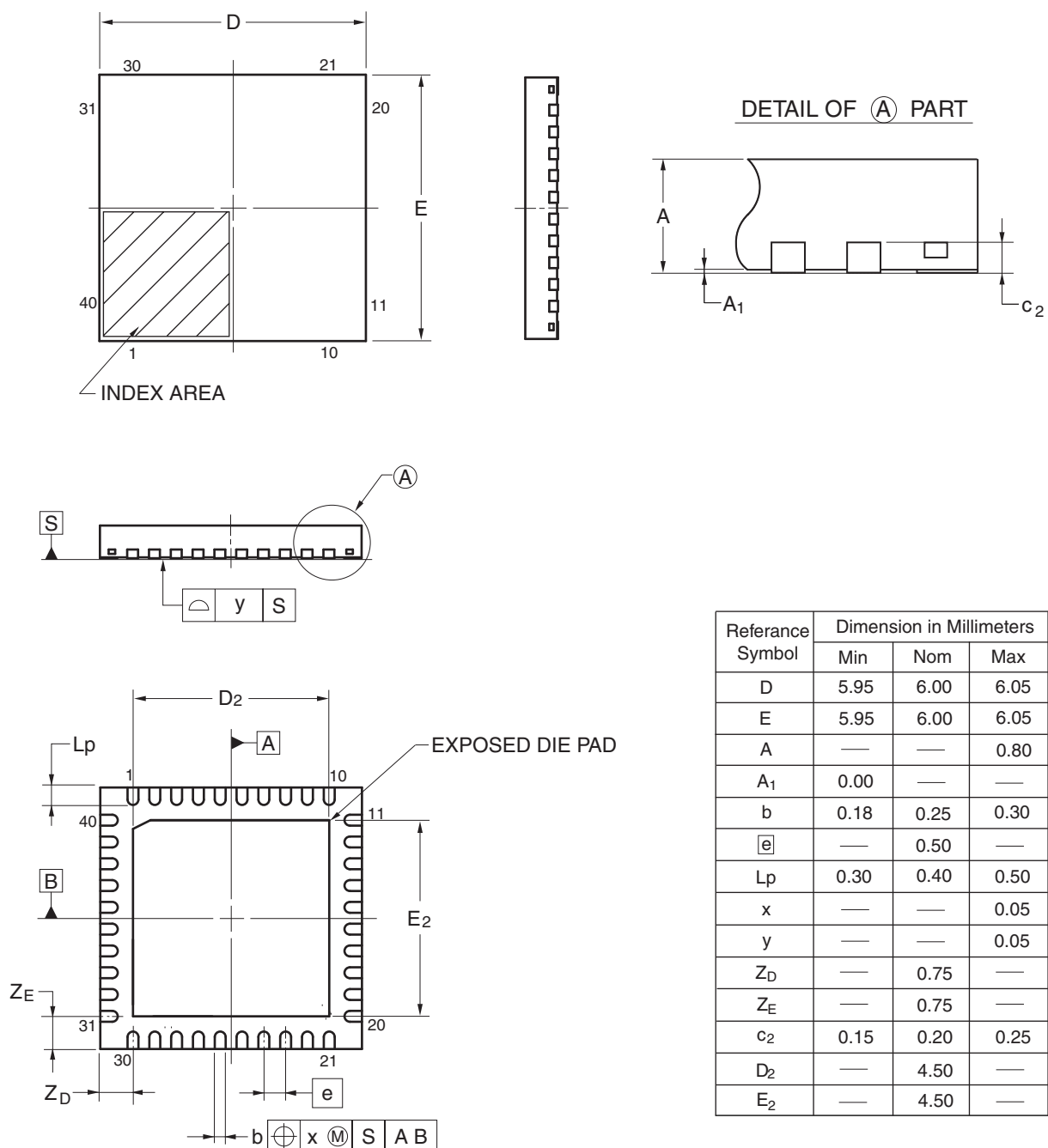
Figure 2.6 QFN 40-pin (1)
