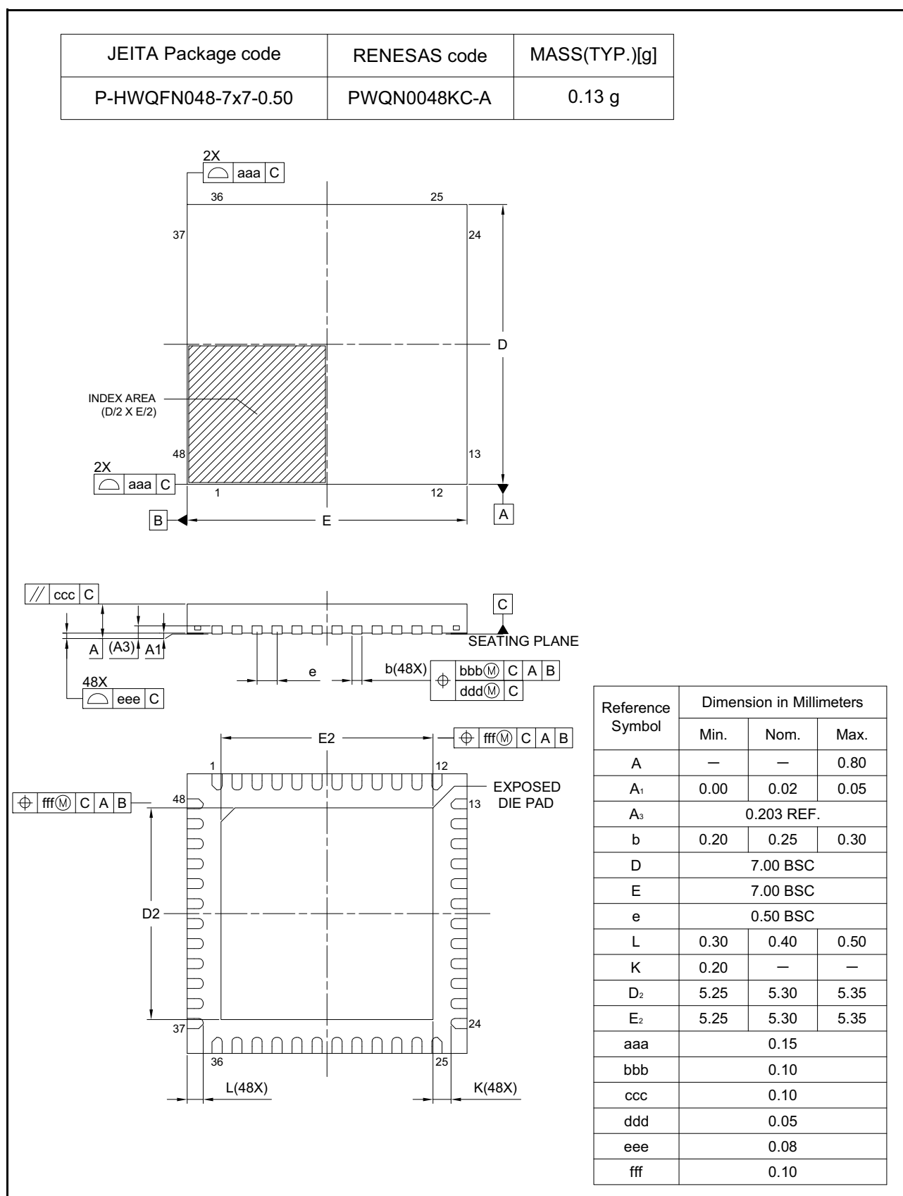
Figure 2.5 QFN 48-pin (2)
