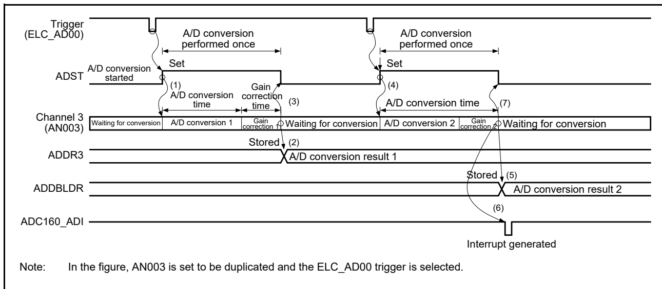
Figure 32.13 Example of operation in single scan mode with double trigger mode selected when AN003 is duplicated
