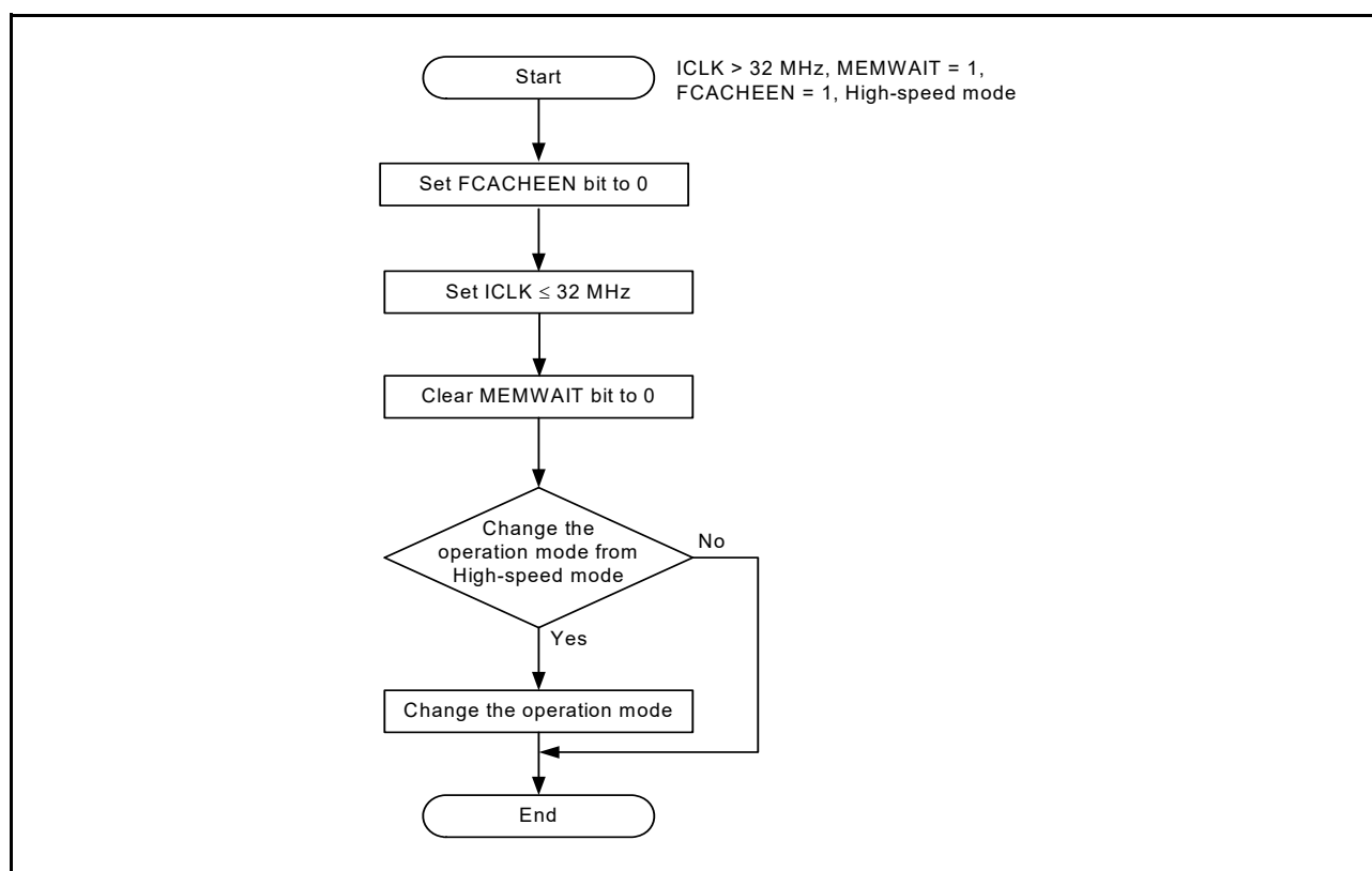
Figure 9.3 When setting the ICLK \leq 32 MHz from ICLK > 32 MHz
