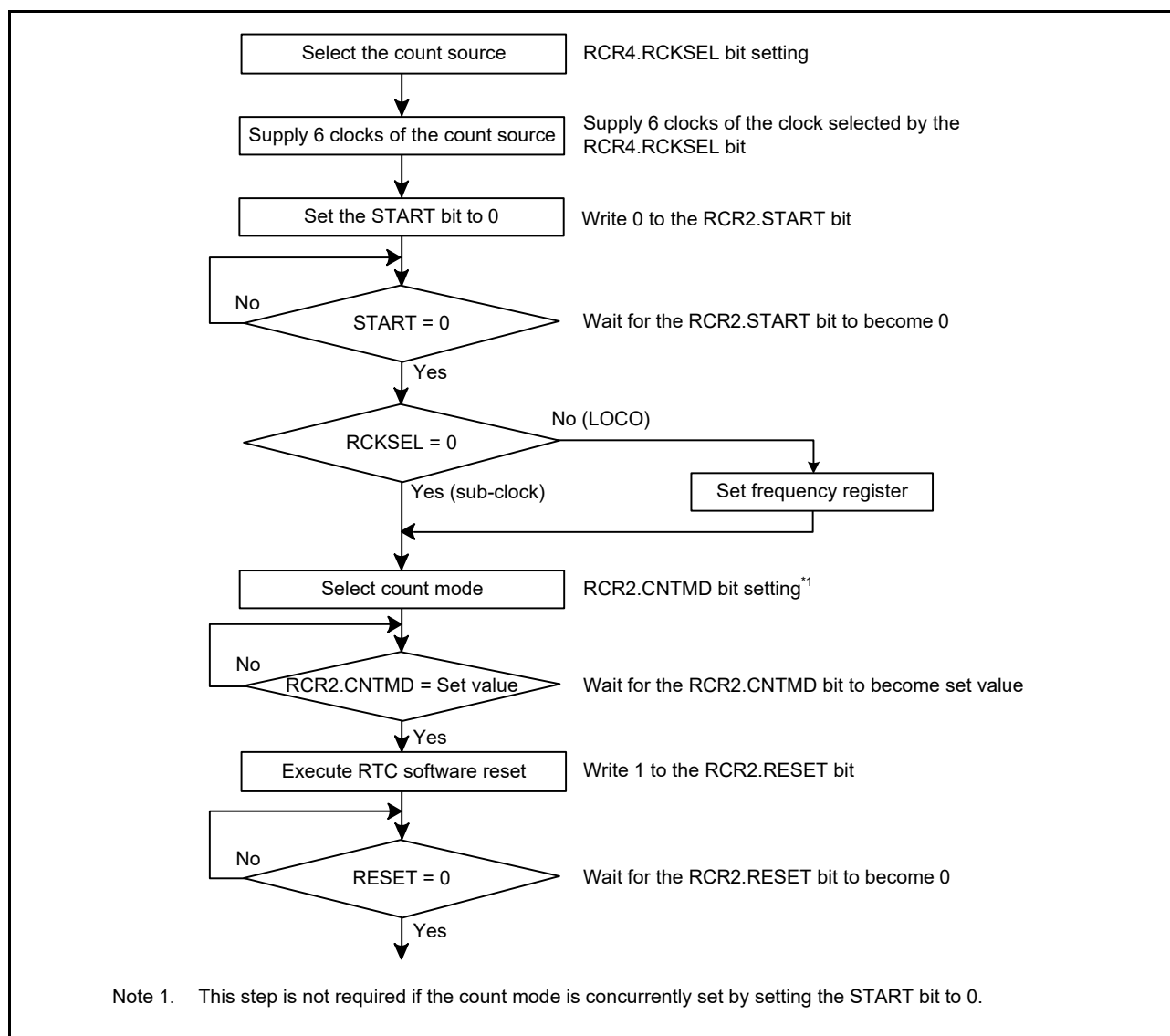
Figure 23.3 Clock and count mode setting procedure
