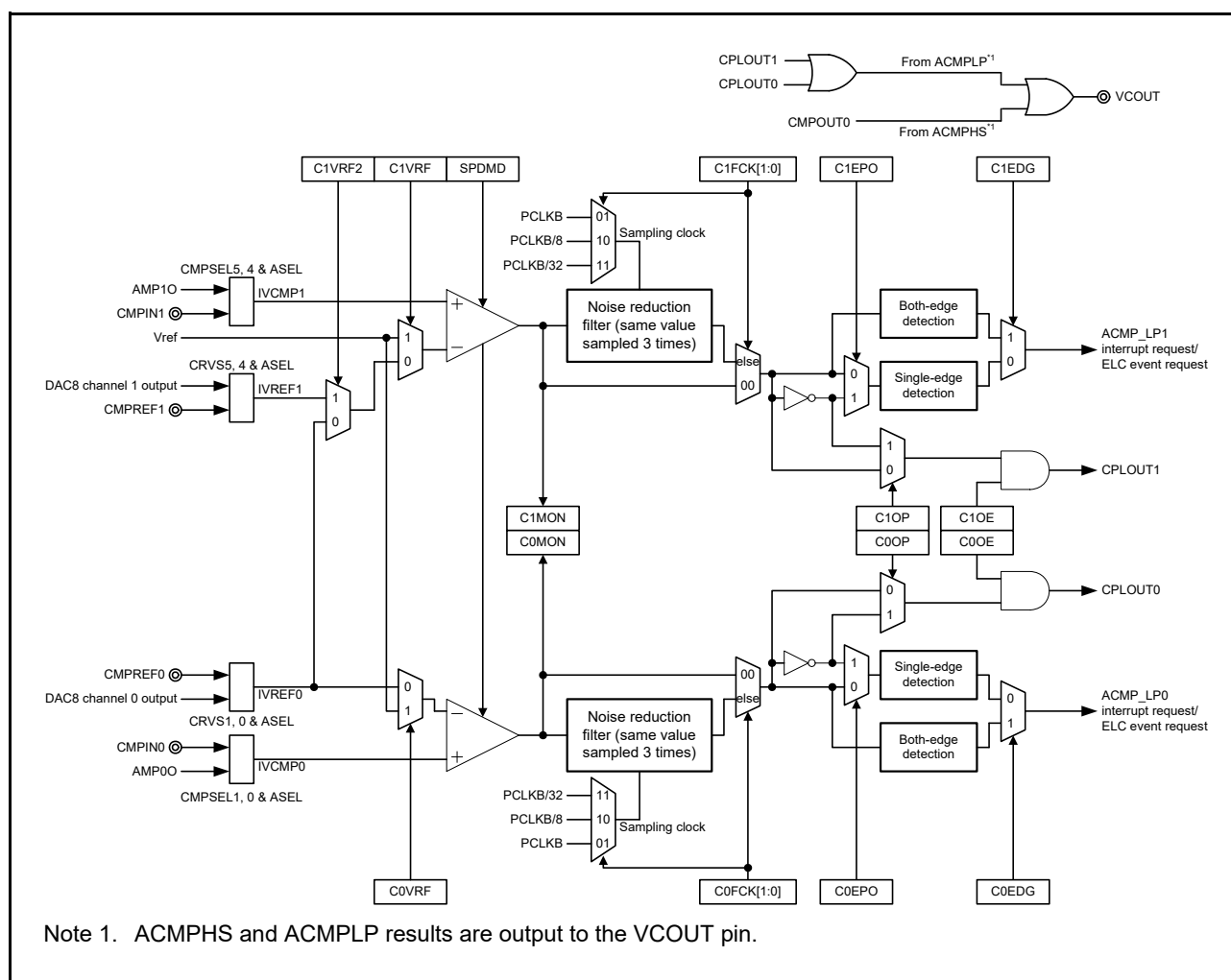
Figure 39.1 ACMLP block diagram when window function is disabled in standard mode
