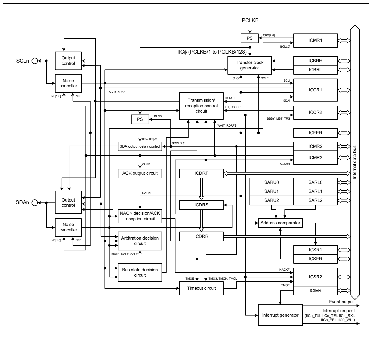
Figure 28.1 IIC block diagram
