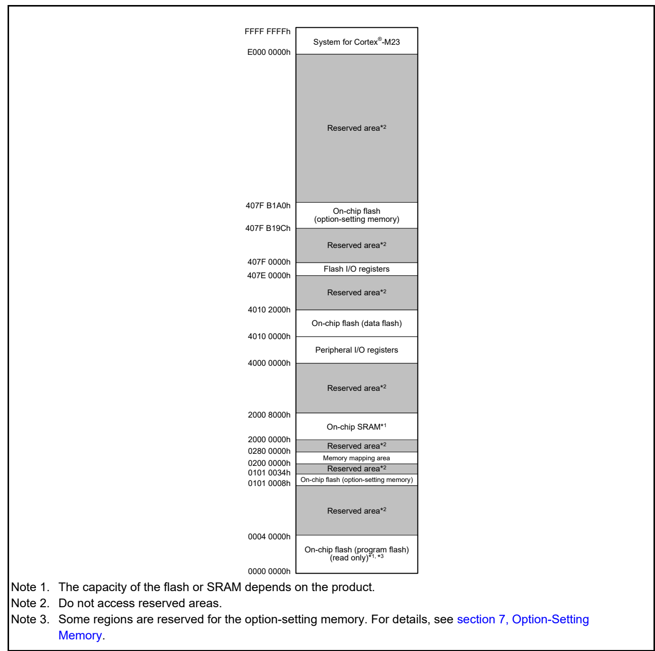
Figure 4.1 Memory map
