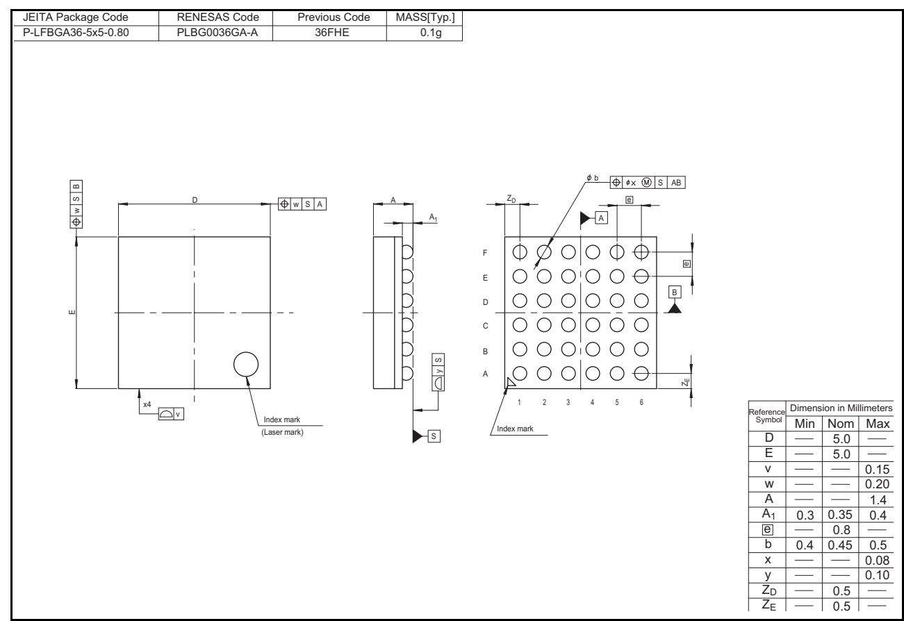
Figure 2.3 BGA 36-pin
