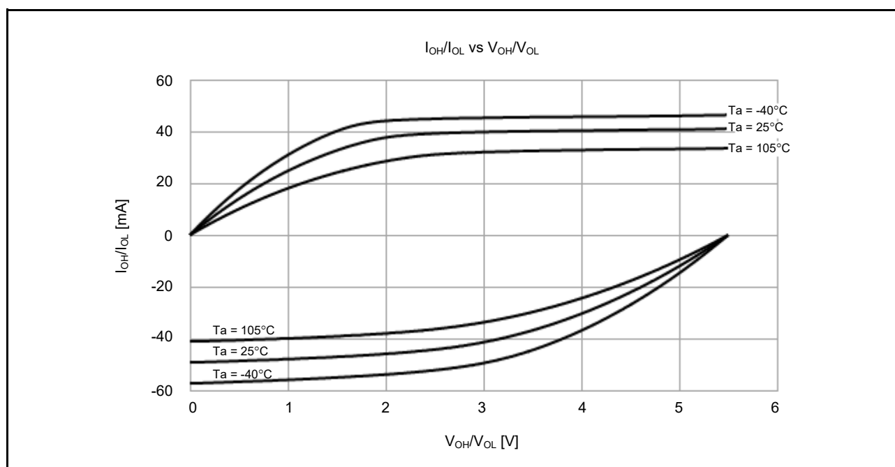
Figure 47.6 V_{OH}/V_{OL} and I_{OH}/I_{OL} temperature characteristics at V_{CC} = 5.5\text{ V} when low drive output is selected (reference data, except for P914 and P915)
