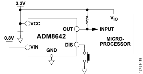
Figure 19. ADM8642 as an Adjustable Threshold Device
