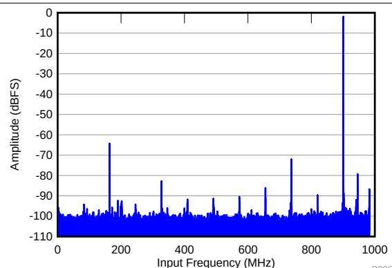
Figure 6. FFT for 900-MHz Input Signal
