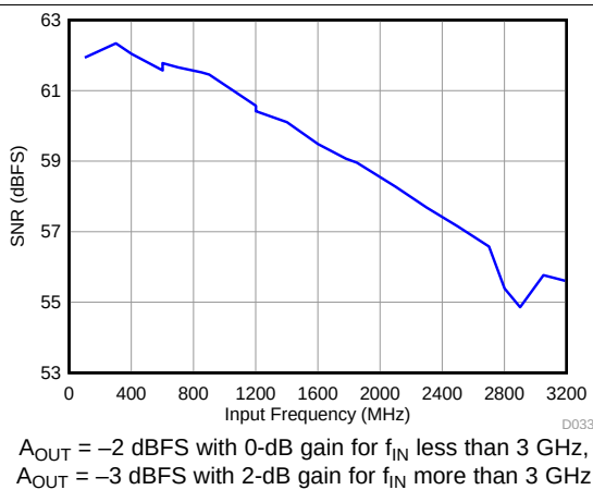
Figure 35. Signal-to-Noise Ratio vs Input Frequency ( f_S = 2211.84 \text{ MSPS} )
