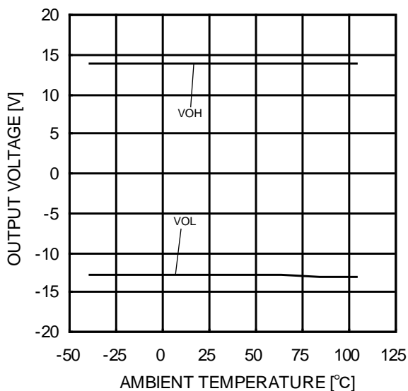
Figure 52. Maximum Output Voltage - Ambient Temperature (VCC/VEE=+15V/-15V, RL=2kΩ)
