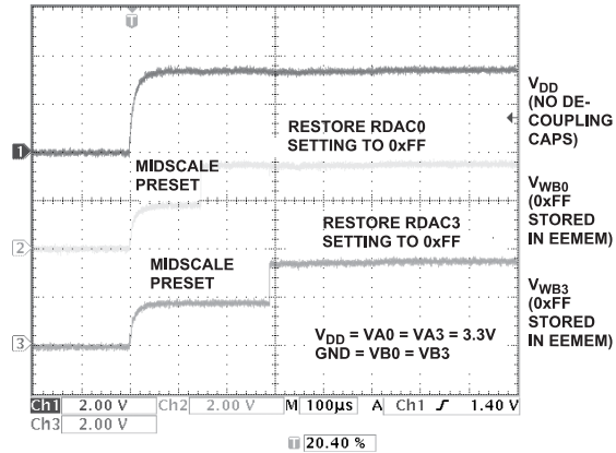
Figure 20. t_{EMEM\_RESTORE} of RDAC0 and RDAC3
