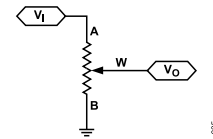
Figure 35. Potentiometer Mode Configuration
