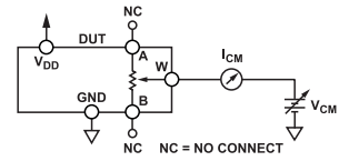
Figure 31. Test Circuit for Common-Mode Leakage Current
