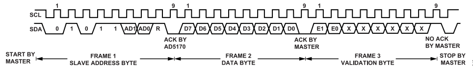
Figure 45. Reading Data from the RDAC Register
