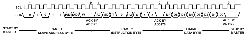
Figure 44. Writing Data to the RDAC Register
