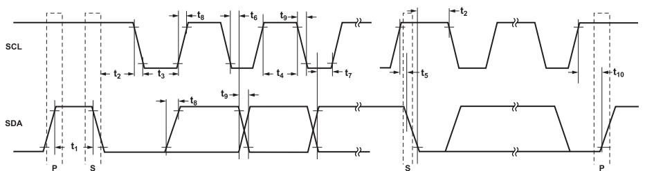
Figure 2. I 2 C Interface Detailed Timing Diagram
