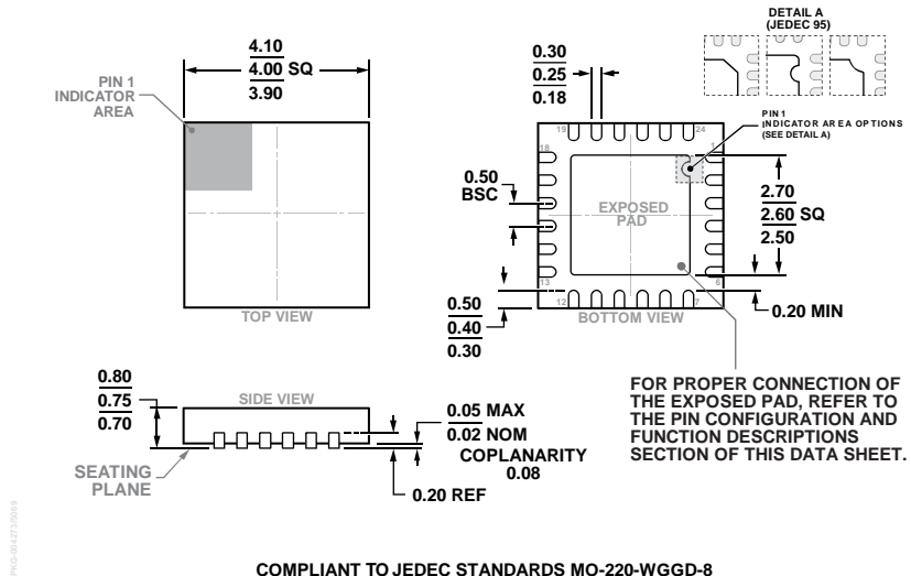
Figure 34. 24-Lead Lead Frame Chip Scale Package [LFCS] 4 mm × 4 mm Body and 0.75 mm Package Height (CP-24-15) Dimensions shown in millimeters
