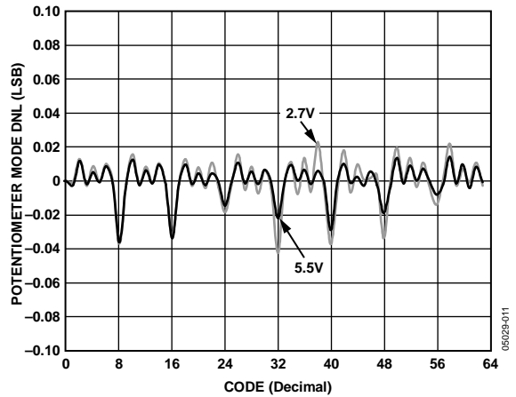
Figure 10. DNL vs. Code vs. Supply Voltages
