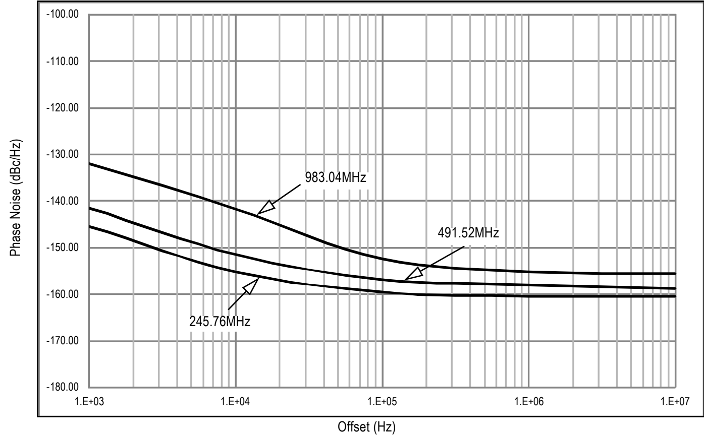
Figure 8. Additive Clock Phase Noise Characteristics (85°C, Worst Case Simulation Model)
