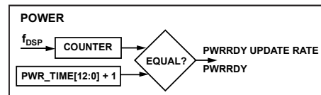
Figure 63. EGYRDY and PWRRDY Update Rates
