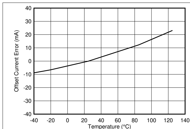
Figure 9-5. Offset Current Error vs Temperature
