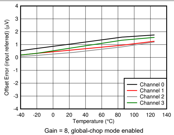
Figure 6-5. Offset Error vs Temperature
