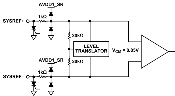
Figure 32. SYSREF± Inputs
