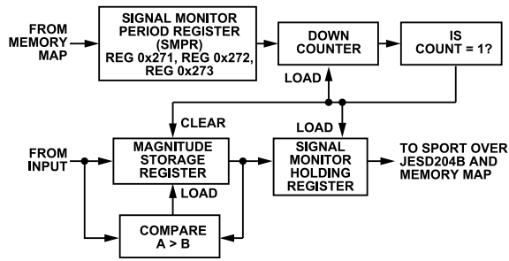
Figure 57. Signal Monitor Block
