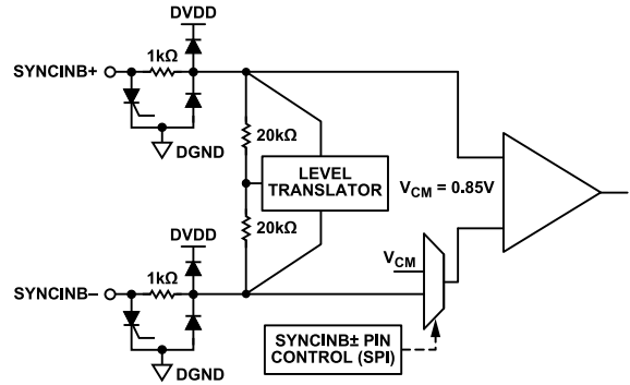
Figure 34. SYNCINB± Inputs
