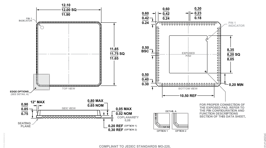
Figure 85. 88-Lead Lead Frame Chip Scale Package [LFCSP] 12 × 12 mm Body and 0.85 mm Package Height (CP-88-4) Dimensions shown in millimeters
