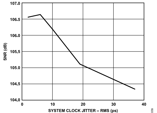
Figure 22. SNR vs. System Clock Jitter, Wideband 0.433 x ODR Filter
