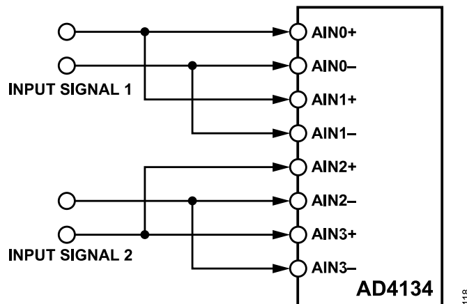
Figure 93. 2:1 Channel Averaging
