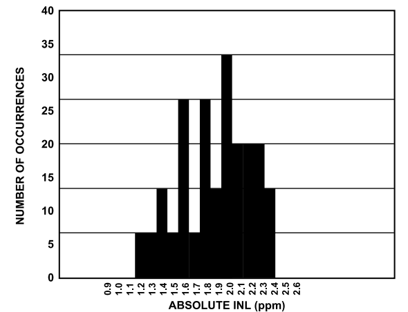
Figure 41. INL Distribution, Wideband 0.433 × ODR Filter, High Performance Mode
