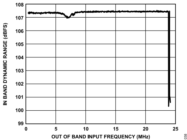
Figure 31. In Band Dynamic Range vs. Out of Band Input Frequency of 1 V p-p Input Signal, Wideband 0.433 x ODR Filter, High Performance Mode
