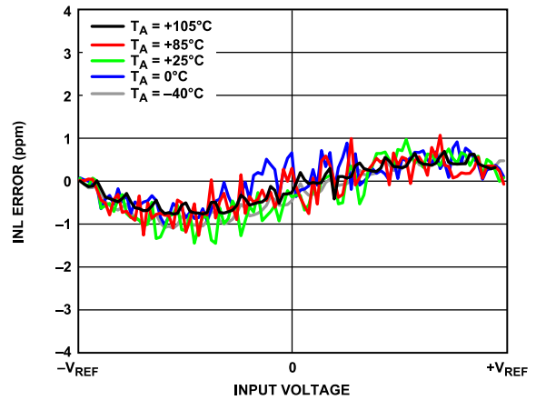
Figure 39. INL Error vs. Input Voltage, Wideband 0.433 × ODR Filter, High Performance Mode
