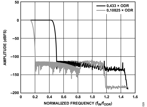
Figure 33. Output Amplitude vs. Normalized Frequency ( f_{IN}/f_{ODR} ), Full Scale Input signal, Wideband 0.433 x ODR Filter, High Performance Mode
