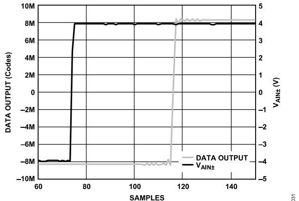
Figure 35. Step Response, Wideband Filter, Wideband 0.433 x ODR Filter
