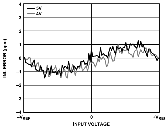
Figure 37. INL Error vs. Input Voltage, Wideband 0.433 × ODR Filter, High Performance Mode
