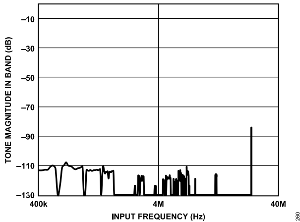
Figure 32. Tone Magnitude In Band vs. Input Frequency, 4 V p-p Input Signal, Wideband 0.433 x ODR Filter, High Performance Mode
