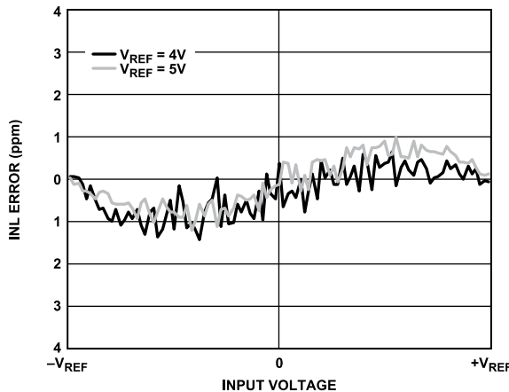
Figure 38. INL Error vs. Input Voltage, Wideband 0.433 × ODR Filter, Low Power Mode
