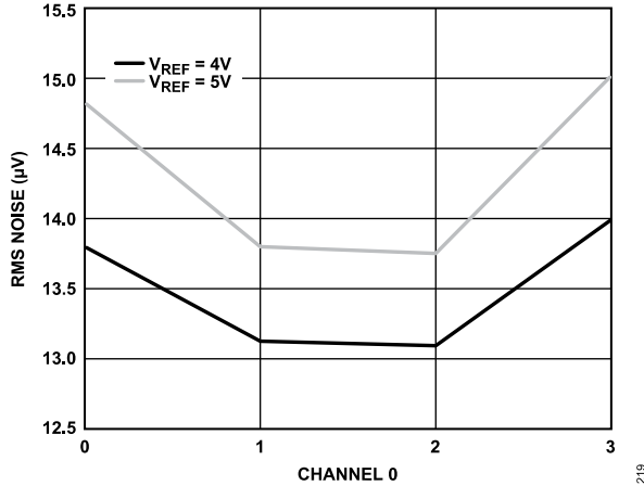
Figure 30. RMS Noise per Channel for Various V_{REF} Values, Wideband 0.433 x ODR Filter, Low Power Mode
