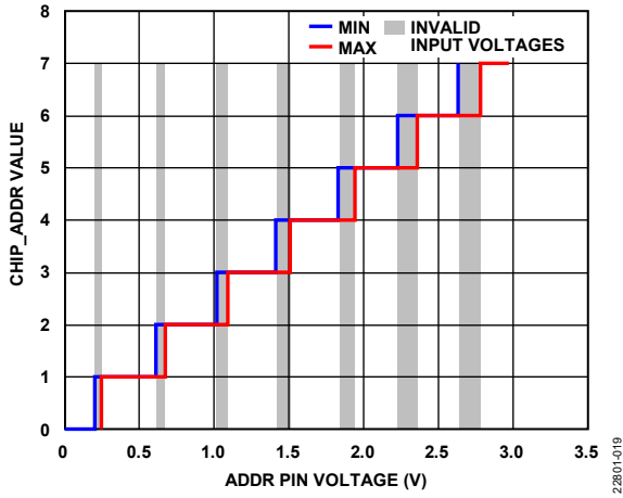
Figure 18. Decoded SPI Address (CHIP_ADDR) Value vs. ADDR Pin Voltage
