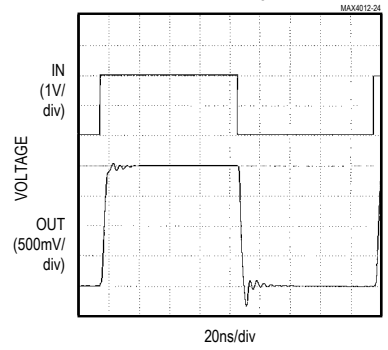
LARGE-SIGNAL PULSE RESPONSE ( C_L = 5pF , A_{VCL} = 2 )
