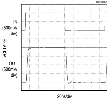
LARGE-SIGNAL PULSE RESPONSE ( A_{VCL} = 2 )
