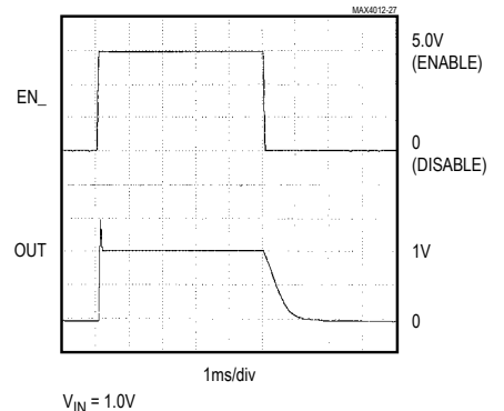
ENABLE RESPONSE TIME
