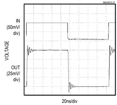
SMALL-SIGNAL PULSE RESPONSE ( C_L = 5pF , A_{VCL} = 1 )
