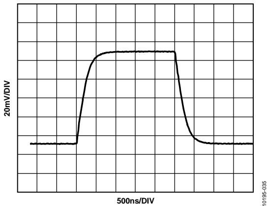
Figure 31. VOVM Small Signal Step Response
