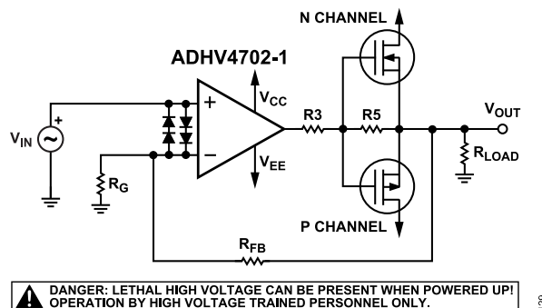
Figure 64. High Current Output Driver Schematic
