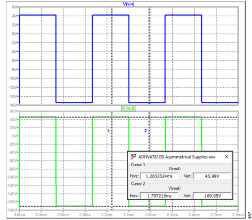
Figure 67. Typical Asymmetrical Supplies Operation Simulation Results
