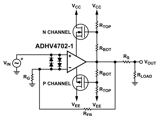
Figure 65. Voltage Extender Schematic
