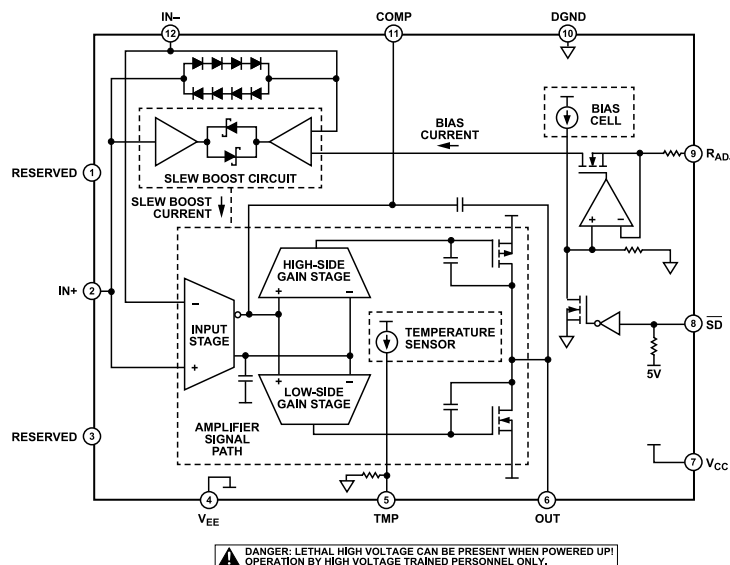
Figure 44. Functional Block Diagram
