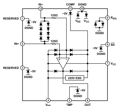
Figure 45. Simplified ESD Configuration
