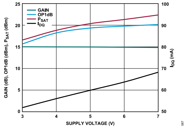
Figure 67. Gain, OP1dB, P SAT , and I DQ vs. Supply Voltage, Power Compression at 5 GHz, R BIAS = 1.43 kΩ
