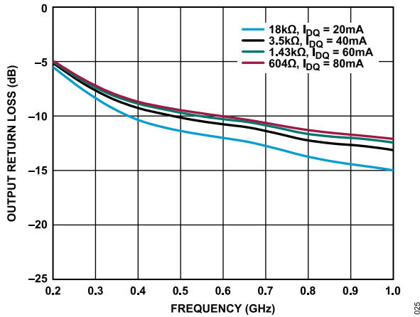
Figure 25. Output Return Loss vs. Frequency for Various Supply Currents, 200 MHz to 1 GHz, V_{DD} = 5\text{ V}
