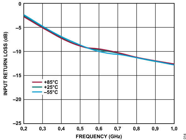
Figure 14. Input Return Loss vs. Frequency for Various Temperatures, 200 MHz to 1 GHz, V DD = 5 V, I DQ = 60 mA
