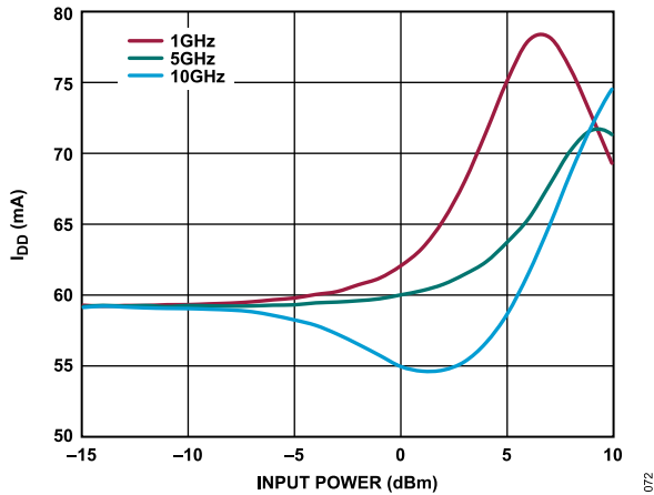
Figure 71. Drain Current (I DD ) vs. Input Power for Various Frequencies, V DD = 5 V, R BIAS = 1.43 kΩ
