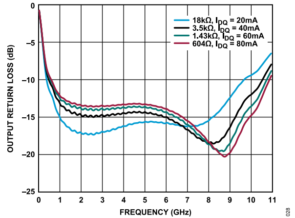
Figure 28. Output Return Loss vs. Frequency for Various Supply Currents, V_{DD} = 5\text{ V}
