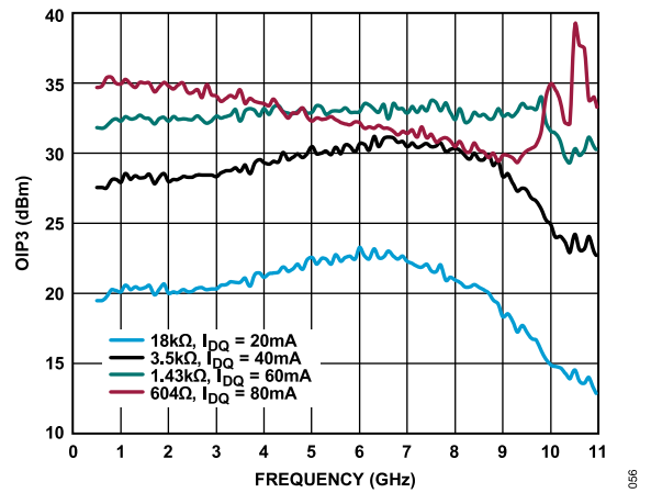
Figure 56. OIP3 vs. Frequency for Various Supply Currents, V_{DD} = 5\text{ V}
