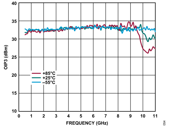
Figure 54. OIP3 vs. Frequency for Various Temperatures, V_{DD} = 5\text{ V} , I_{DQ} = 60\text{ mA} , P_{OUT} = 0\text{ dBm} per Tone
