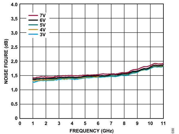
Figure 30. Noise Figure vs. Frequency for Various Supply Voltages, I_{DQ} = 60\text{ mA}
