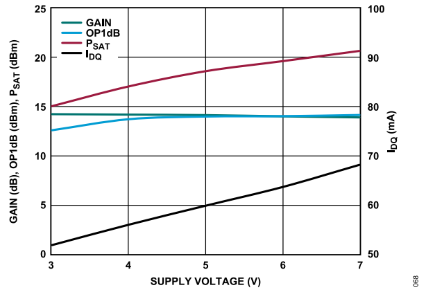
Figure 68. Gain, OP1dB, P SAT , and I DQ vs. Supply Voltage, Power Compression at 10 GHz, R BIAS = 1.43 kΩ
