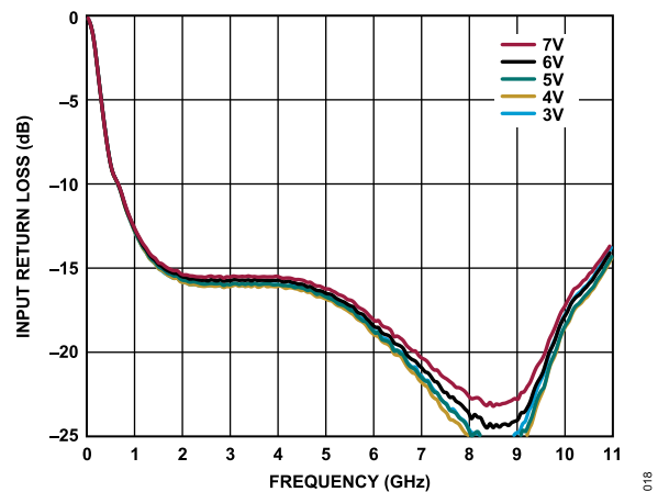
Figure 18. Input Return Loss vs. Frequency for Various Supply Voltages, I DQ = 60 mA
