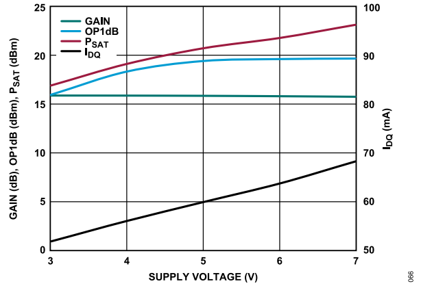
Figure 66. Gain, OP1dB, P SAT , and I DQ vs. Supply Voltage, Power Compression at 1 GHz, R BIAS = 1.43 kΩ
