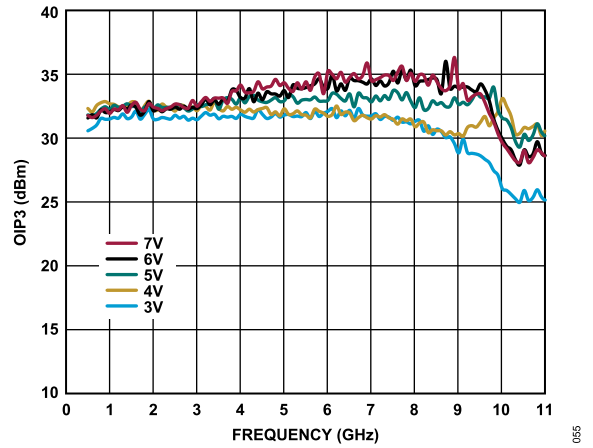
Figure 55. OIP3 vs. Frequency for Various Supply Voltages, I_{DQ} = 60\text{ mA}
