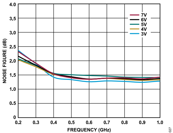
Figure 27. Noise Figure vs. Frequency for Various Supply Voltages, 200 MHz to 1 GHz, I_{DQ} = 60\text{ mA}
