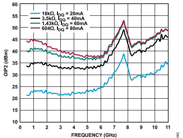
Figure 62. OIP2 vs. Frequency for Various Supply Currents, V_{DD} = 5\text{ V}
