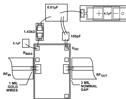
Figure 75. Assembly Diagram
