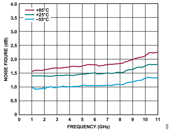
Figure 29. Noise Figure vs. Frequency for Various Temperatures, V_{DD} = 5\text{ V} , I_{DQ} = 60\text{ mA}
