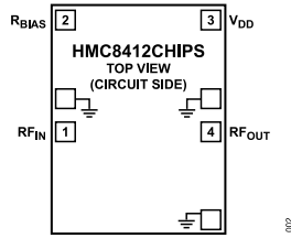
Figure 2. Pad Configuration
