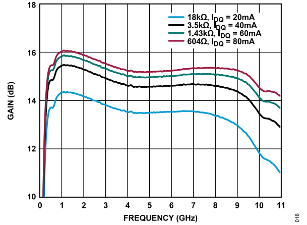
Figure 16. Gain vs. Frequency for Various Supply Currents, V DD = 5 V
