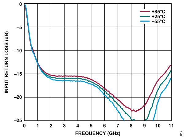
Figure 17. Input Return Loss vs. Frequency for Various Temperatures, V DD = 5 V, I DQ = 60 mA
