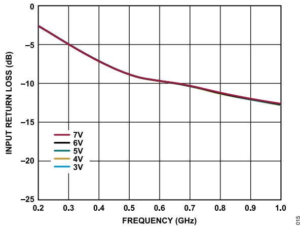
Figure 15. Input Return Loss vs. Frequency for Various Supply Voltages, 200 MHz to 1 GHz, I DQ = 60 mA
