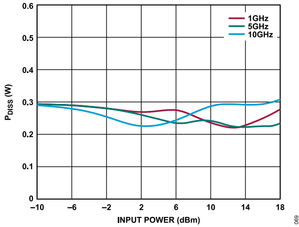
Figure 69. P DISS vs. Input Power at T A = 85°C, V DD = 5 V, I DQ = 60 mA
