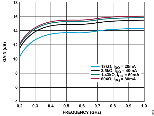
Figure 13. Gain vs. Frequency for Various Supply Currents, 200 MHz to 1 GHz, V DD = 5 V
