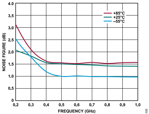
Figure 26. Noise Figure vs. Frequency for Various Temperatures, 200 MHz to 1 GHz, V_{DD} = 5\text{ V} , I_{DQ} = 60\text{ mA}
