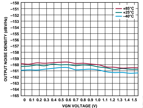
Figure 77. Output Noise Density vs. VGN Voltage over Temperature at 3 GHz
