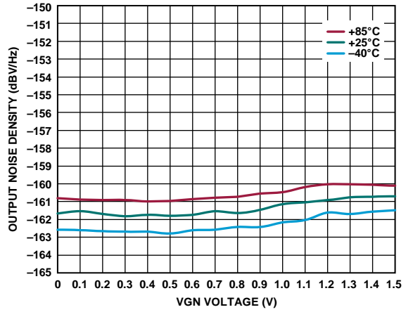
Figure 75. Output Noise Density vs. VGN Voltage over Temperature at 1 GHz
