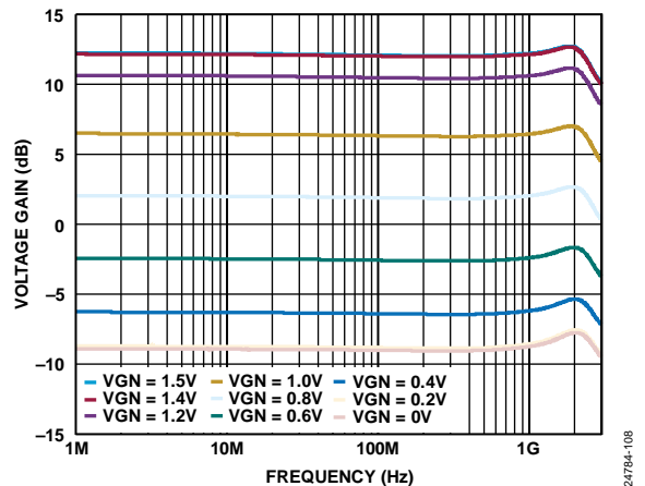
Figure 8. Voltage Gain vs. Frequency over 200 mV VGN Steps, 43 Ω Back Terminations not De-Embedded
