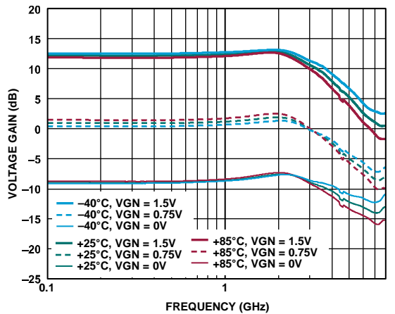
Figure 62. Voltage Gain vs. Frequency, over Temperature and VGN, 43 Ω Back Terminations not De-Embedded
