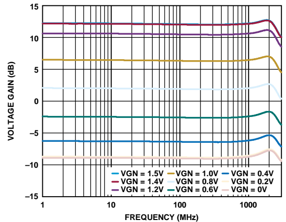
Figure 65. Voltage Gain vs. Frequency over 200 mV VGN Steps, 43 Ω Back Terminations not De-Embedded
