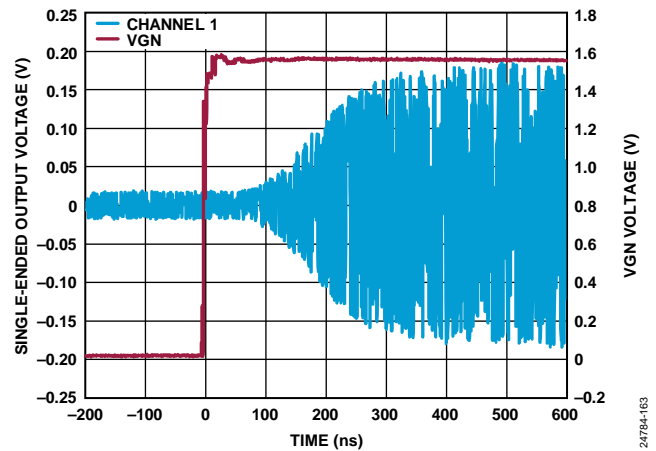
Figure 56. VGA Step Response Rise Time, Minimum to Maximum Gain
