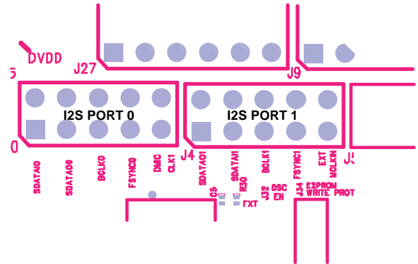
Figure 32. Serial Audio Port
