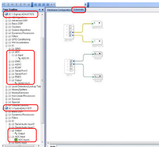
Figure 16. AIN2 and AIN3 Inputs to SDSP OUT1 and SDSP OUT2 , AIN0 and AIN1 Inputs to FDSP Output1 and Output2
