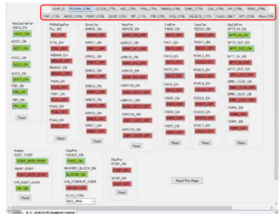
Figure 18. ADAU1787 POWER_CTRL Tab (Register Control)
