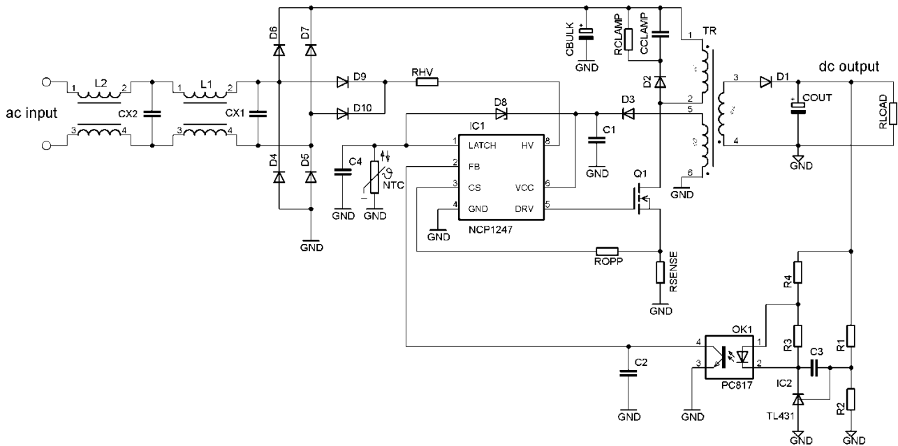
Figure 1. Flyback Converter Application Using the NCP1247
