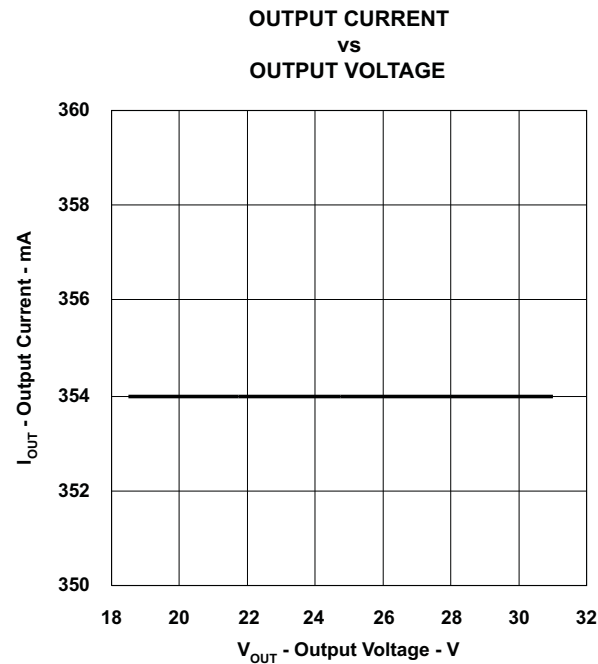
Figure 7. Load Regulation
