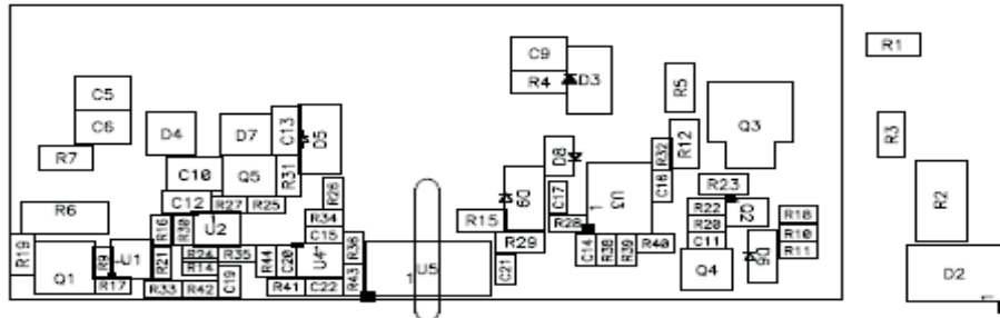
Figure 17. Bottom Assembly Drawing (bottom view)
