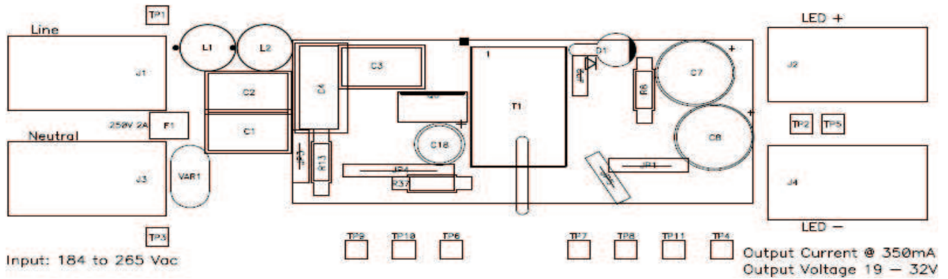
Figure 16. Top Layer Assembly Drawing (top view)
