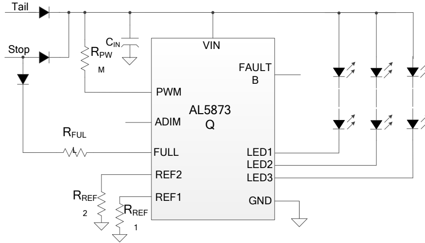
Figure 1. Typical Application
