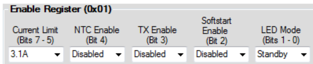
Figure 17. Enable Register
