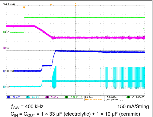
Figure 8-4. Typical Start-Up
