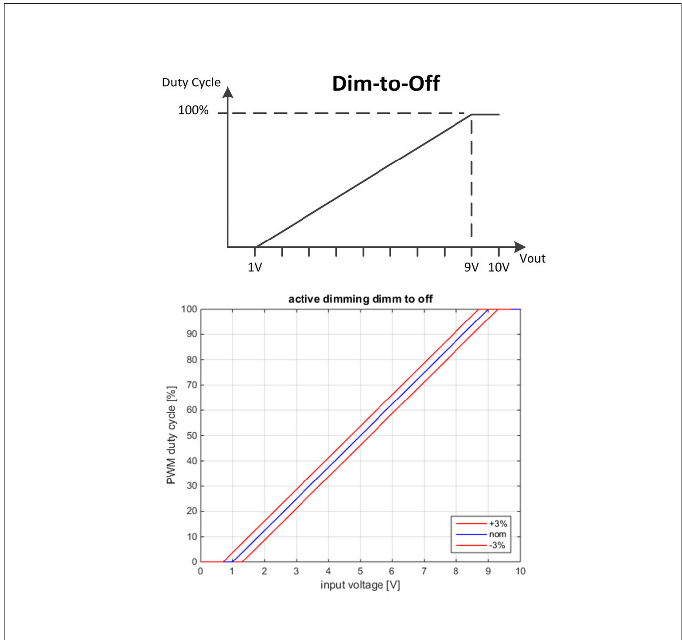
Figure 4 Dimming Characteristic
