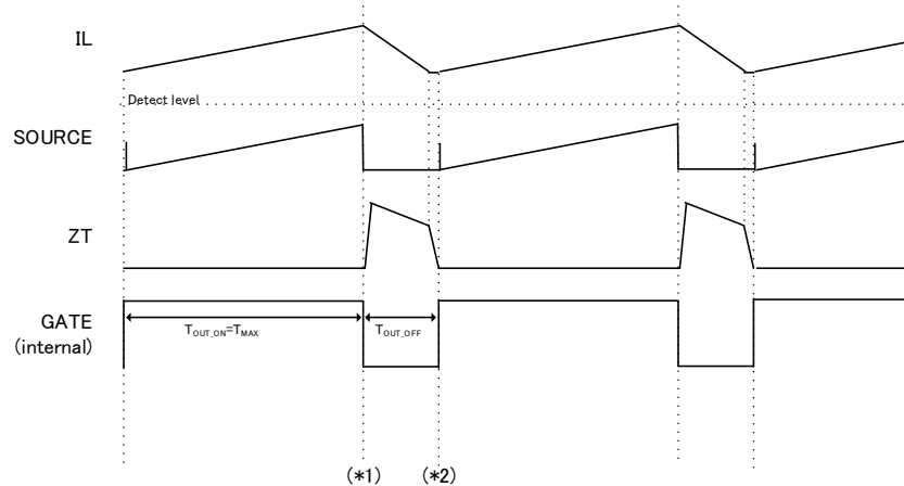
Figure 12. Maximum On time operation waveform
