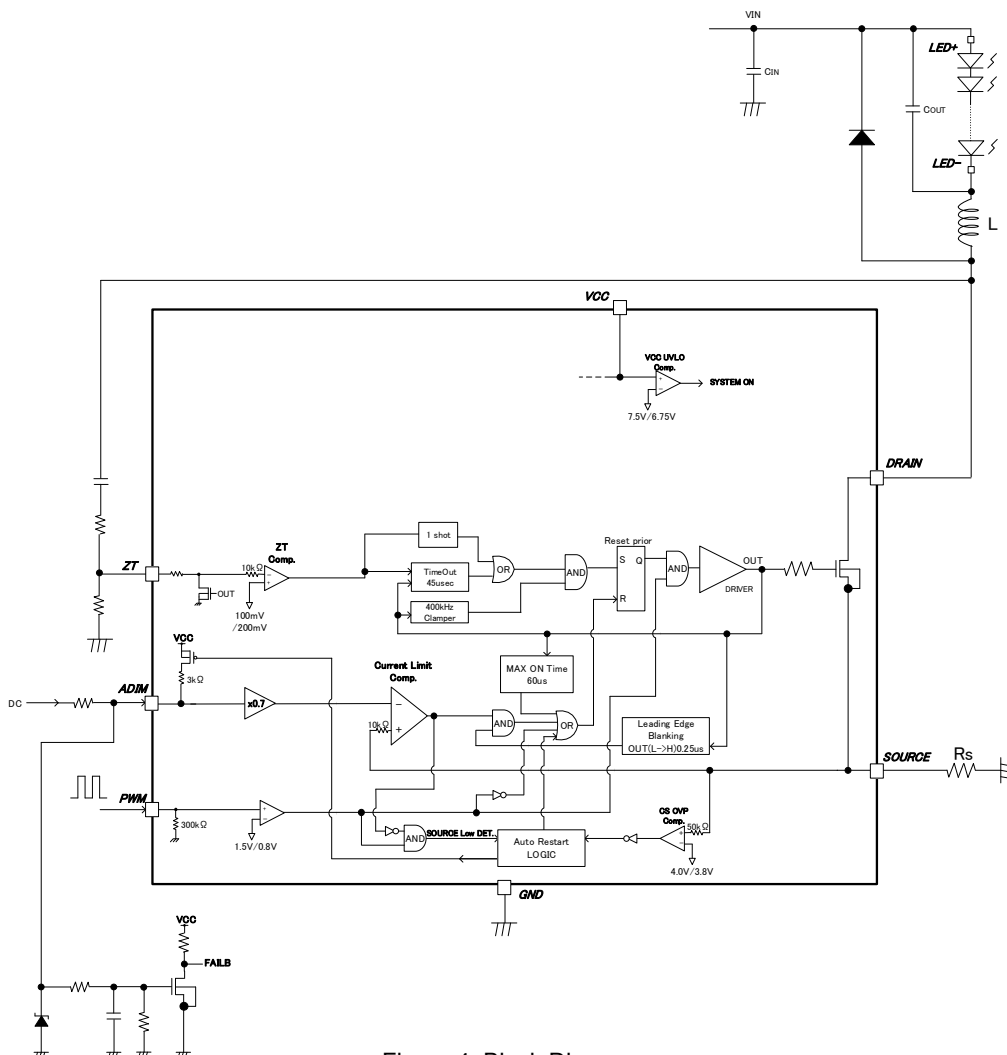
Figure 4. Block Diagram
