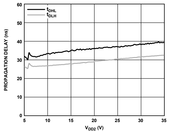
Figure 15. Propagation Delay vs. V_{DD2} , 2\text{ nF} Load
