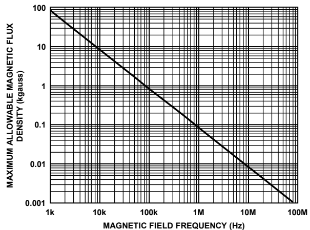
Figure 24. Maximum Allowable External Magnetic Flux Density
