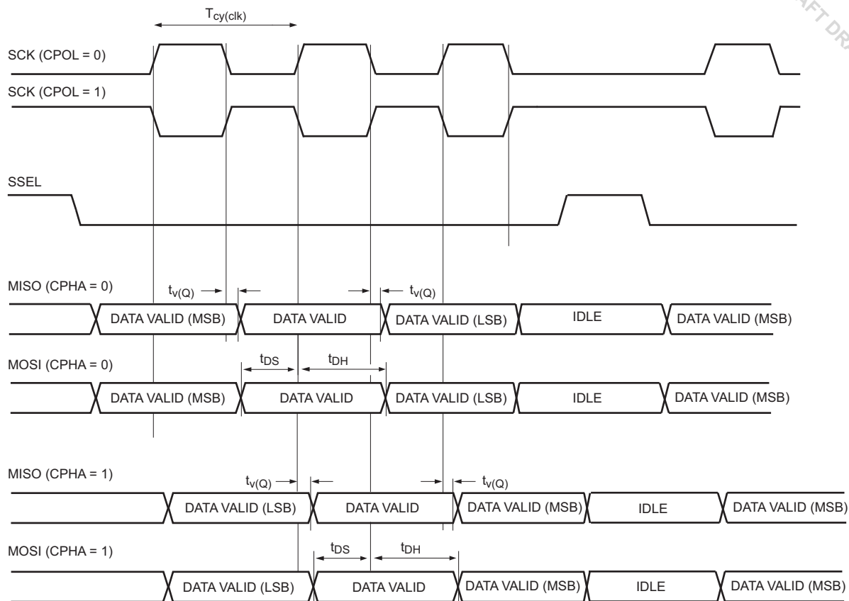
Fig 35. SPI slave timing
