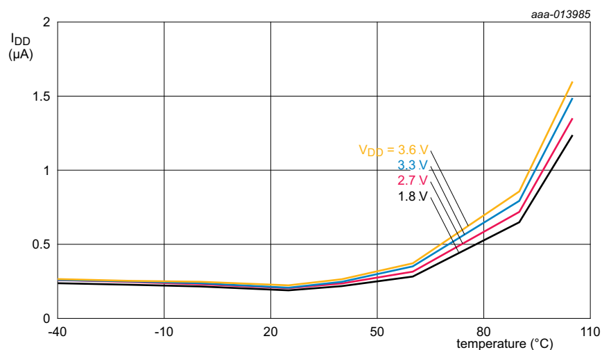
Fig 18. Deep power-down mode: Typical supply current I_{DD} versus temperature for different supply voltages V_{DD}
