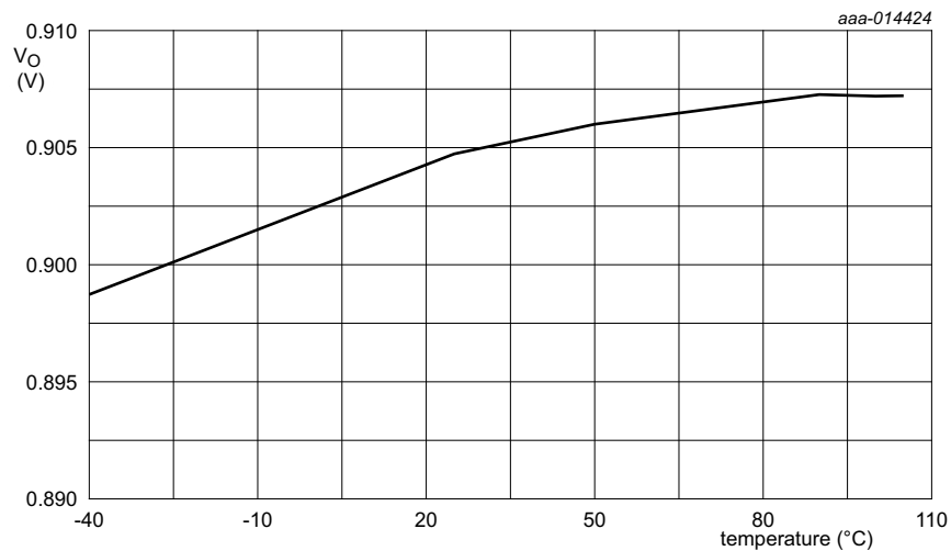
Fig 39. Typical internal voltage reference output voltage
