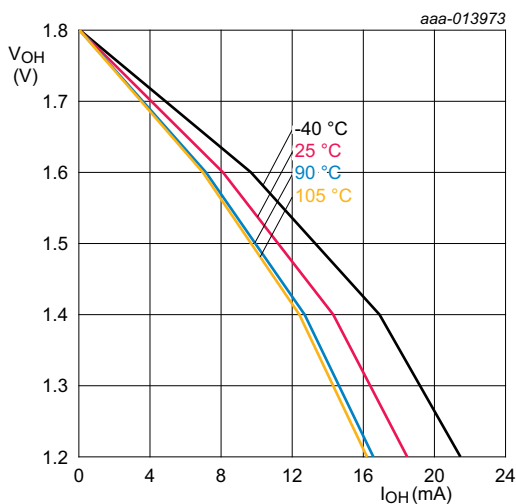
Fig 25. High-drive output: Typical HIGH-level output voltage V_{OH} versus HIGH-level output current I_{OH}
