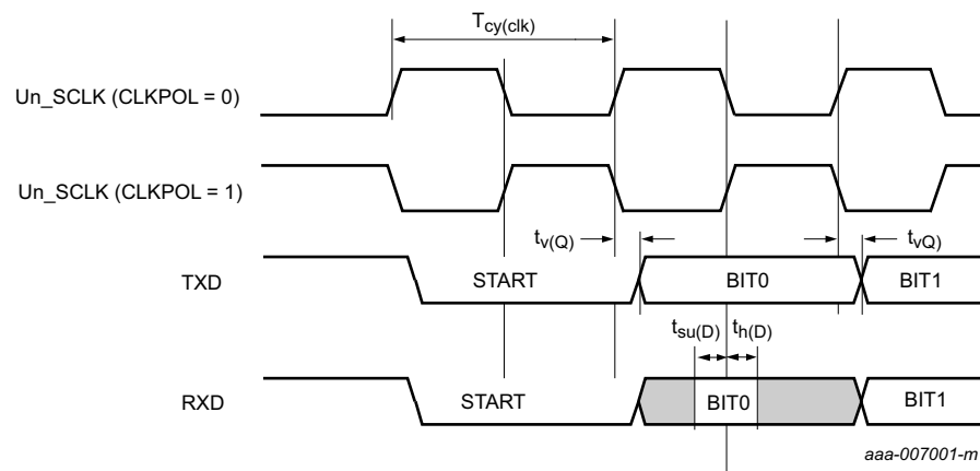
Fig 36. USART timing
