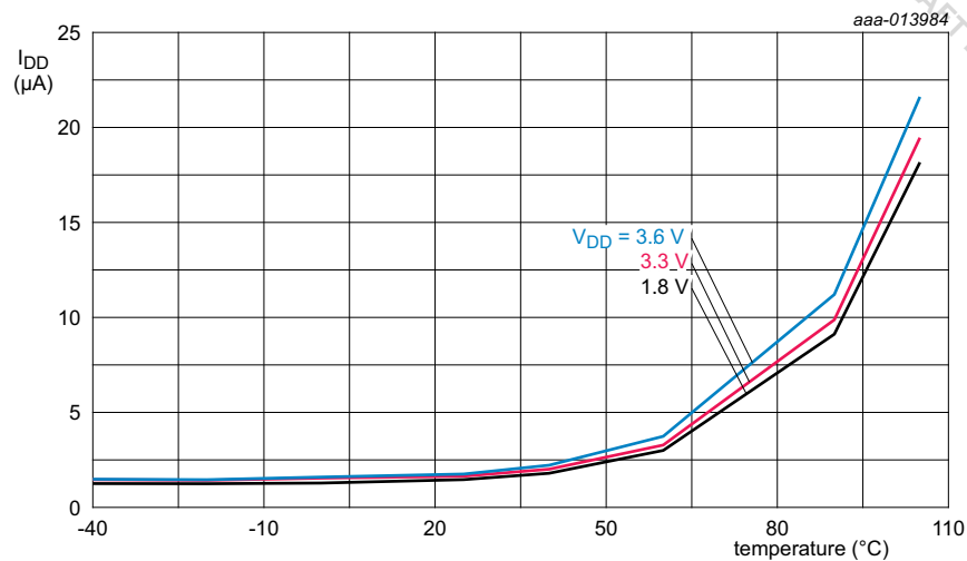
Fig 17. Power-down mode: Typical supply current I_{DD} versus temperature for different supply voltages V_{DD}
