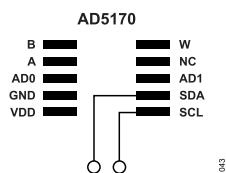
Figure 43. Recommended AD5170 PCB Layout
