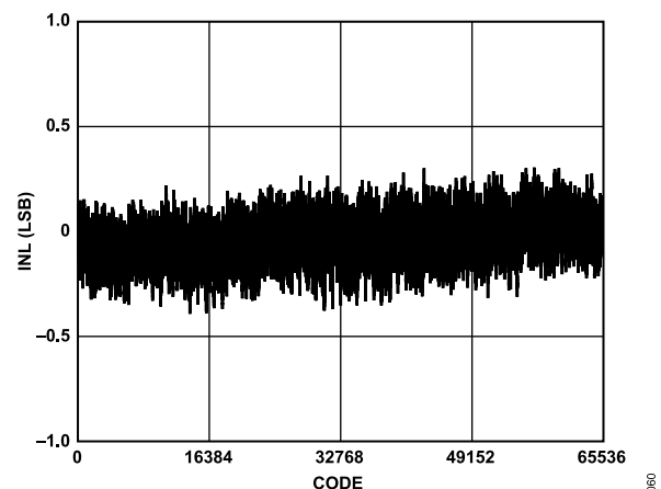
Figure 66. Integral Nonlinearity
