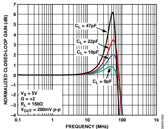
Figure 30. Small-Signal Frequency Response vs. C_L , ADA4891-3/ADA4891-4
