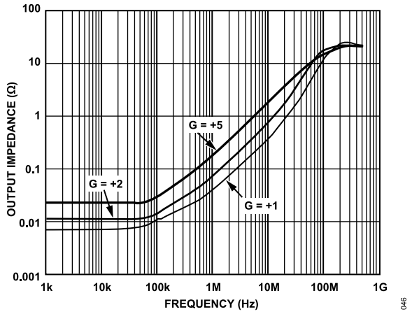
Figure 51. Output Enabled—Impedance vs. Frequency
