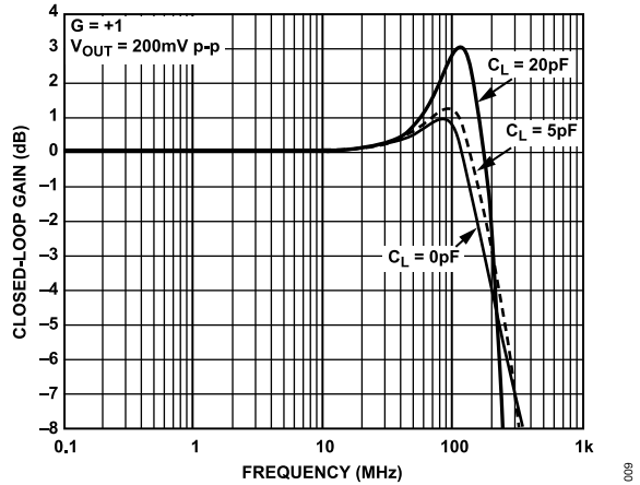
Figure 14. AD8027 Small Signal Frequency Response for Various C_{LOAD} Values
