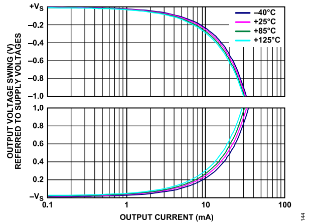
Figure 44. Operational Amplifier Output Voltage Swing vs. Output Current, V_S = 3 V
