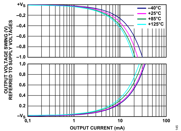
Figure 45. Operational Amplifier Output Voltage Swing vs. Output Current, V_S = 5 V
