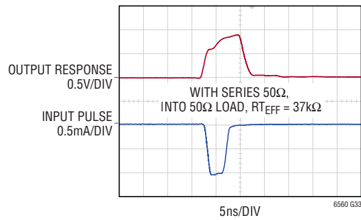
Pulse Response Overload Region (1mA)
