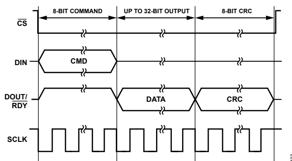
Figure 123. SPI Read Transaction with CRC
