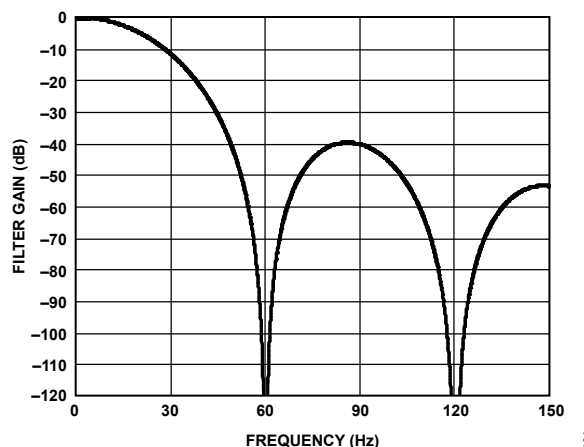
Figure 94. \text{Sinc}^3 Filter Response (60 SPS Output Data Rate, Zero Latency Disabled or 20 SPS Output Data Rate, Zero Latency Enabled)
