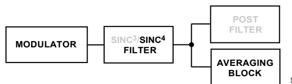
Figure 97. Fast Settling Mode, Sinc 4 + Sinc 1 Filter
