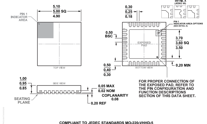
Figure 130. 32-Lead Lead Frame Chip Scale Package [LFCSP] 5 mm x 5 mm Body and 0.95 mm Package Height (CP-32-30) Dimensions shown in millimeters
