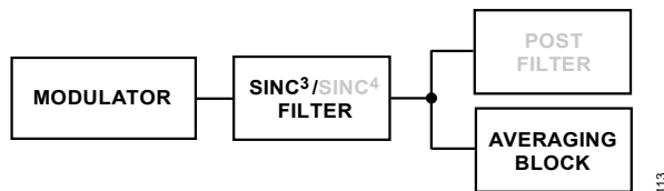
Figure 103. Fast Settling Mode, \text{Sinc}^3 + \text{Sinc}^1 Filter
