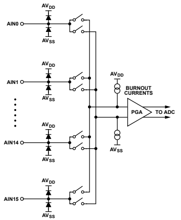
Figure 73. Analog Input Multiplexer Circuit
