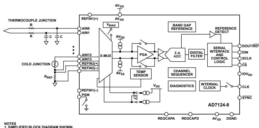
Figure 126. Thermocouple Application
