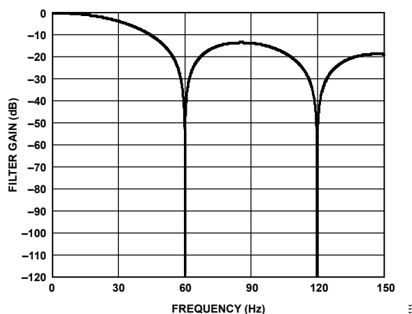
Figure 101. 60 Hz Rejection
