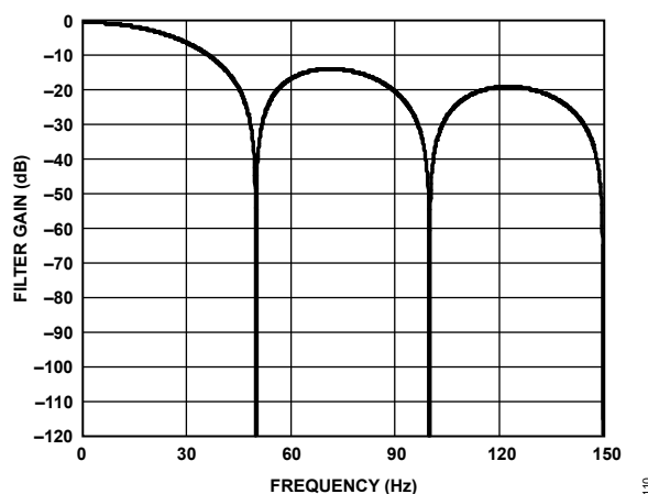
Figure 100. 50 Hz Rejection
