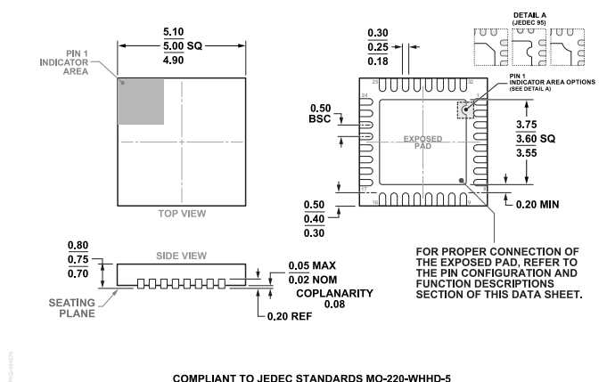
Figure 129. 32-Lead Lead Frame Chip Scale Package [LFCSP] 5 mm x 5 mm Body and 0.75 mm Package Height (CP-32-12) Dimensions shown in millimeters
