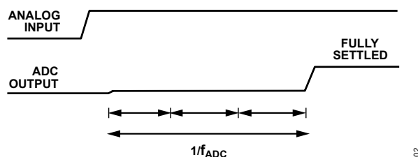
Figure 92. \text{Sinc}^3 Zero Latency Operation
