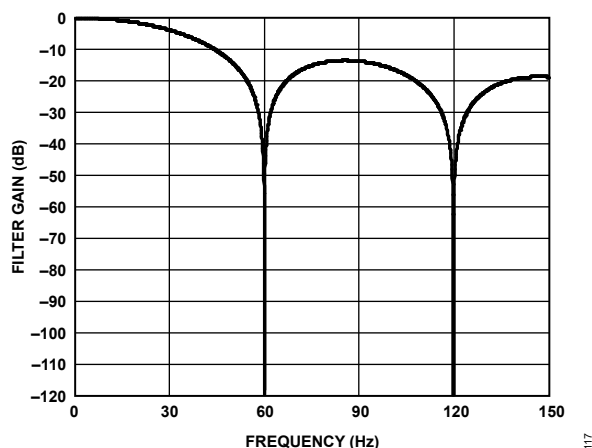
Figure 107. 60 Hz Rejection
