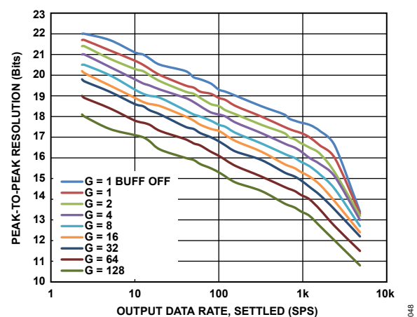
Figure 48. Peak-to-Peak Resolution vs. Output Data Rate (Settled), \text{Sinc}^4 Filter (Full Power Mode)
