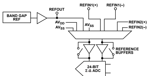
Figure 75. Reference Connections
