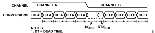
Figure 104. Fast Settling, \text{Sinc}^3 + \text{Sinc}^1 Filter
