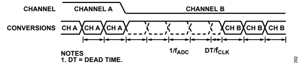
Figure 82. Sinc 4 Channel Change
