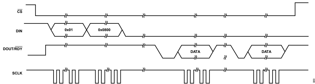
Figure 80. Continuous Read Configuration
