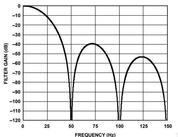
Figure 93. \text{Sinc}^3 Filter Response (50 SPS Output Data Rate, Zero Latency Disabled or 16.67 SPS Output Data Rate, Zero Latency Enabled)
