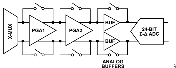
Figure 74. PGA
