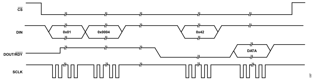
Figure 78. Single Conversion Configuration
