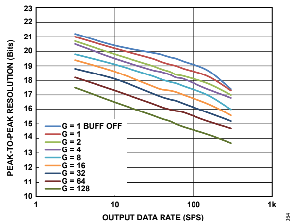
Figure 54. Peak-to-Peak Resolution vs. Output Data Rate, \text{Sinc}^4 + \text{Sinc}^1 Filter (Mid Power Mode)
