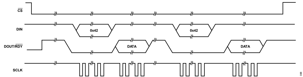
Figure 79. Continuous Conversion Configuration
