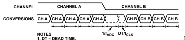
Figure 98. Fast Settling, Sinc 4 + Sinc 1 Filter
