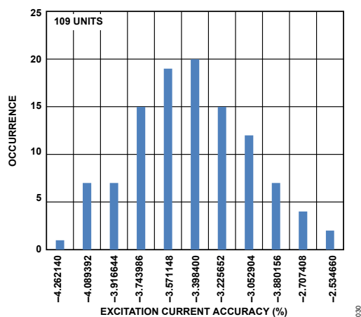
Figure 30. IOUTx Current Initial Accuracy Histogram (500 \mu A)
