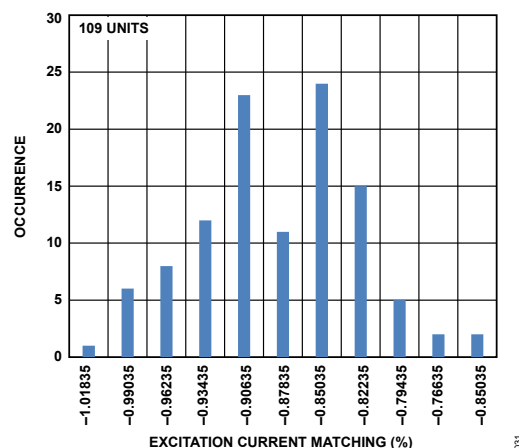
Figure 31. IOUTx Current Initial Matching Histogram (500 \mu A)
