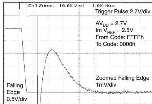
FULL-SCALE SETTLING TIME: 2.7V FALLING EDGE
