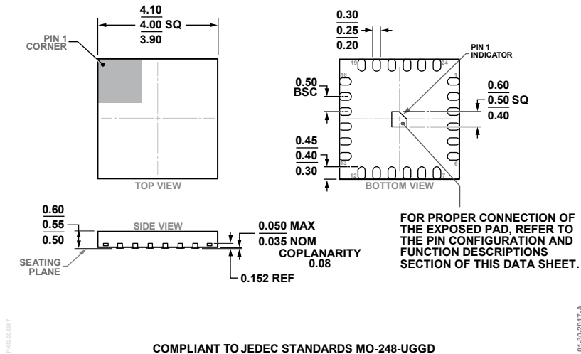
Figure 45. 24-Lead Lead Frame Chip Scale Package [LFCSP] 4 mm × 4 mm Body and 0.55 mm Package Height (CP-24-25)
