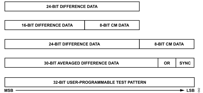
Figure 40. Summary of Selectable Output Sample Formats
