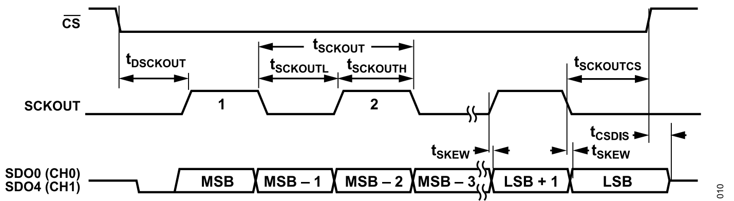
Figure 10. Master Clock Mode Timing, DDR, 1-Lane
