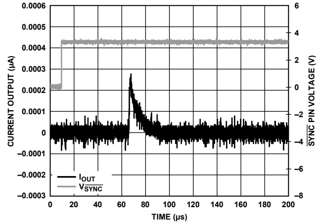
Figure 18. Current Output ( I_{OUT} ) and \overline{SYNC} Pin Voltage ( V_{\overline{SYNC}} ) vs. Time on Output Enable
