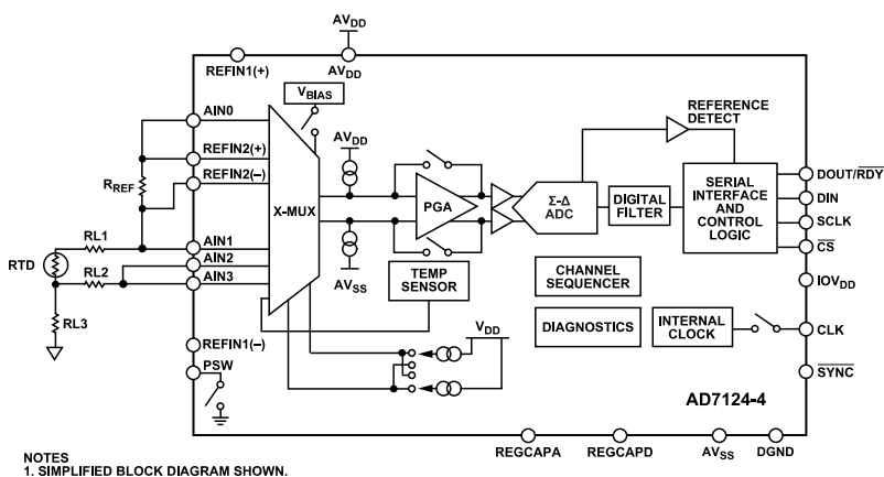
Figure 128. 3-Wire RTD Application
