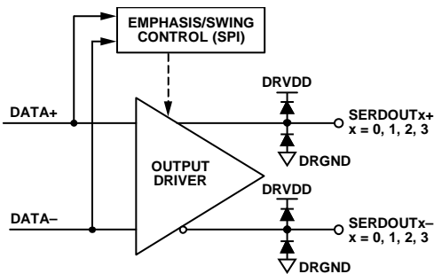
Figure 66. Digital Outputs
