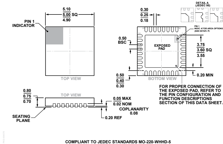
COMPLIANT TO JEDEC STANDARDS MO-220-WHHD-5 Figure 61. 32-Lead Lead Frame Chip Scale Package [LFCS 1 P] 5 mm × 5 mm Body and 0.75 mm Package Height (CP-32-12) Dimensions shown in millimeters
